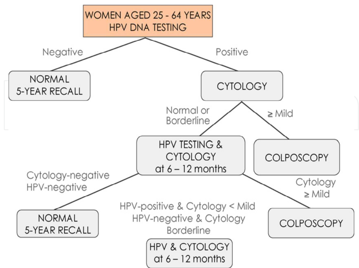
Fig. 6. Proposed new screening algorithm which employs HPV DNA testing as the primary screening test and uses cytology to triage HPV positive women (Cuzick et al., 2008).
