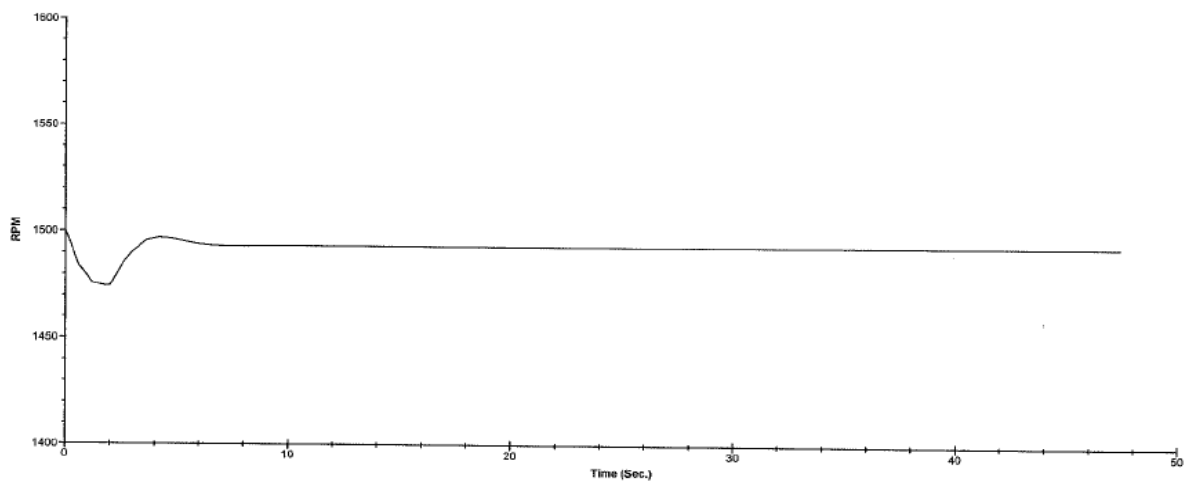
Fig. 12. Speed response after load shedding
