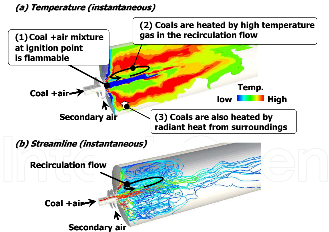
Fig. 2. Examples of detailed calculated results of pulverized coal combustion.
