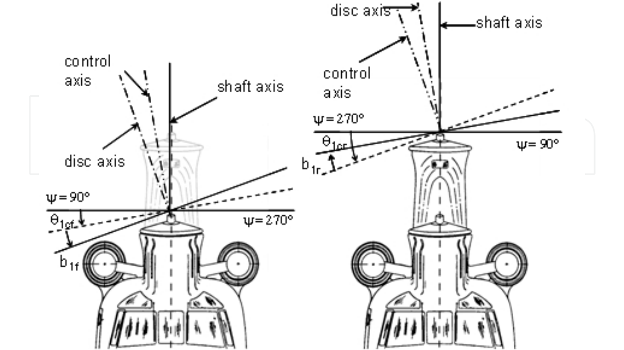
Fig. A4. Lateral axis Chinook control (front view)
