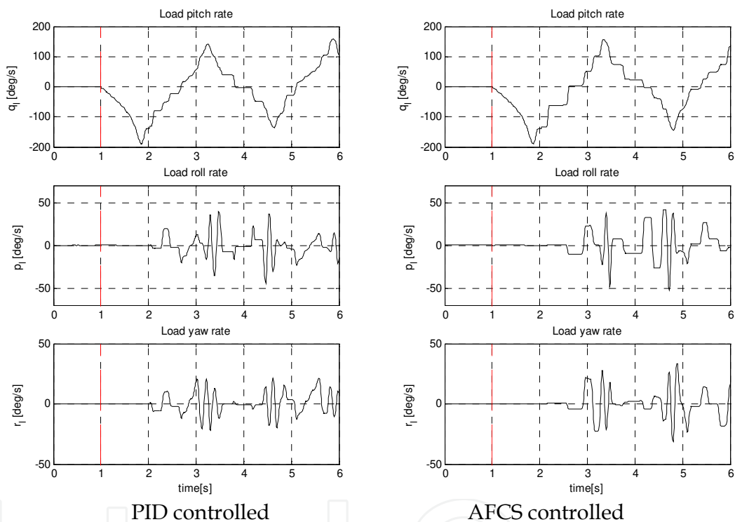
Fig. 11. Load motion after front suspension cable failure
