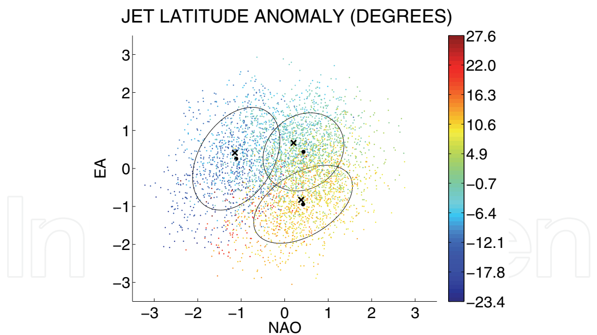
Fig. 6. Scatter plot of the daily winter (DJF) Z500 anomalies, projected onto the NAO/EA plane and color-coded to show the jet latitude. The ellipses and their associated centres correspond respectively to the covariances and the means of the Gaussian component mixture model. The crosses represent the regimes obtained from the jet latitude PDF projected onto the same plane (reproduced from WO10b).
