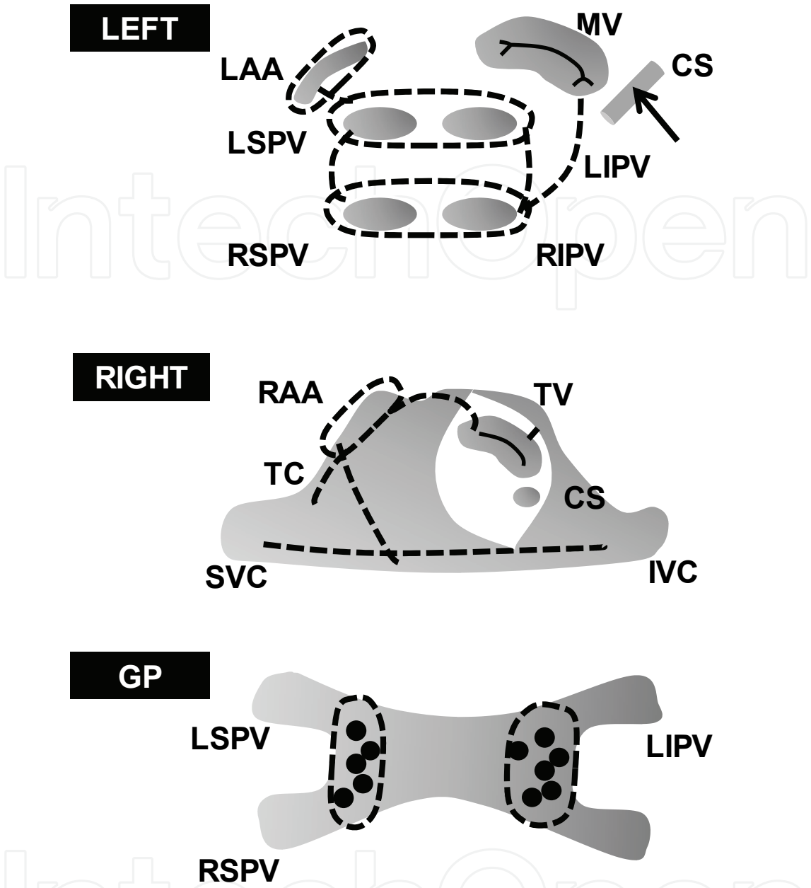
Fig. 2. Illustration of lesion sets for Cox-Maze IV and GP ablation. We illustrate left and right Maze IV lesions (dotted lines) as well as foci for GP (black circles) ablation.
