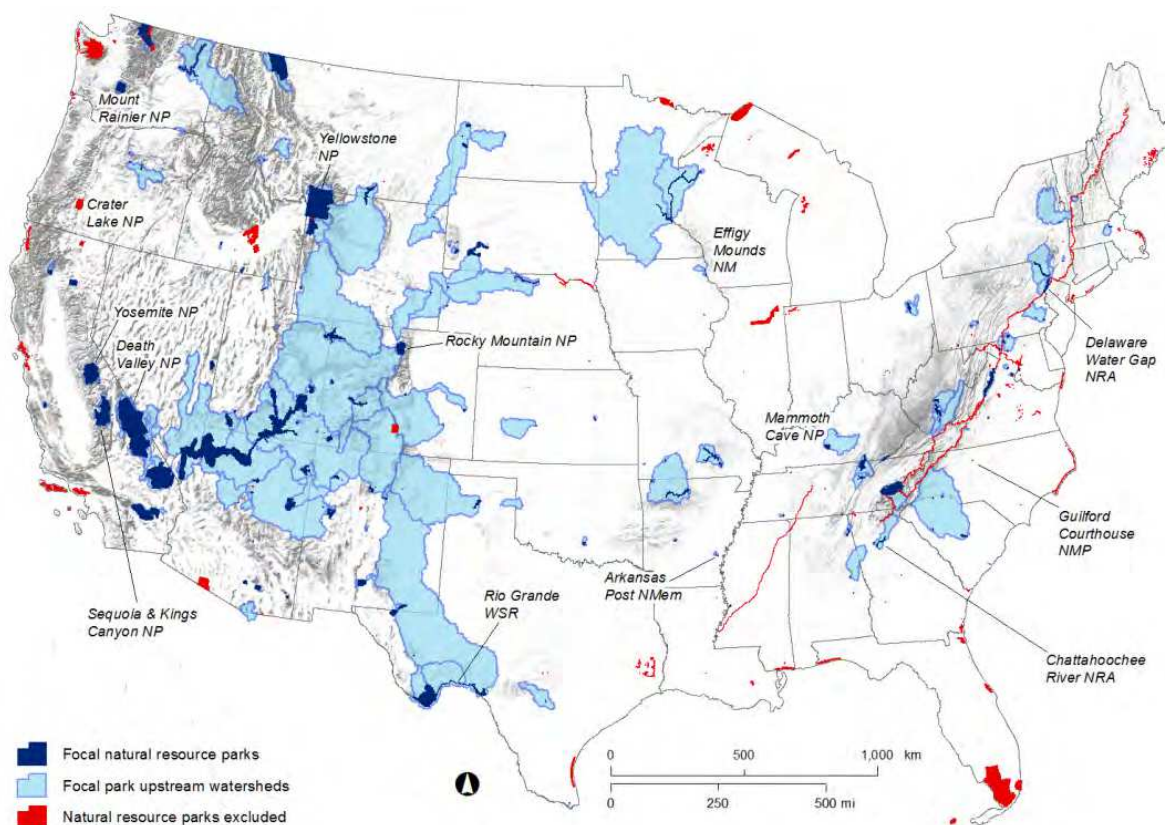
Fig. 2. Focal parks and upstream watersheds considered in the present analyses. Labelled parks are referred to in the text. NP = National Park, NRA = National Recreation Area, NMP = National Military Park, NM = National Monument, NMem = National Memorial, WSR = Wild and Scenic River.
