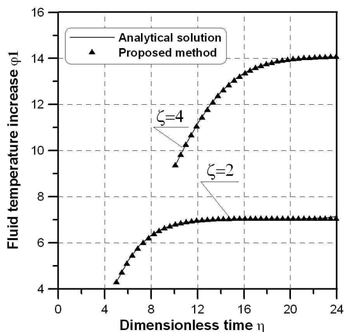
Fig. 7. Histories of dimensionless fluid temperature increase
