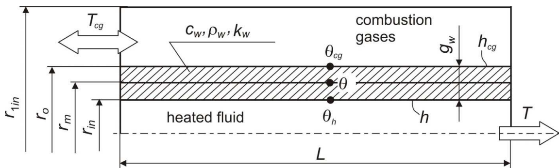
Fig. 2. Tube wall divided into two control volumes
