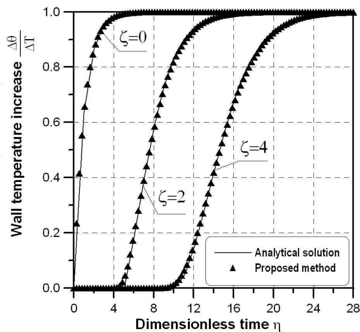
Fig. 6. Dimensionless histories of tube wall temperature increase
