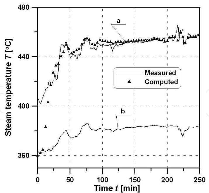
Fig. 11. Comparison of the measured and computed steam temperatures at the superheater outlet (a) and history of the measured steam temperature at the superheater inlet (b)
