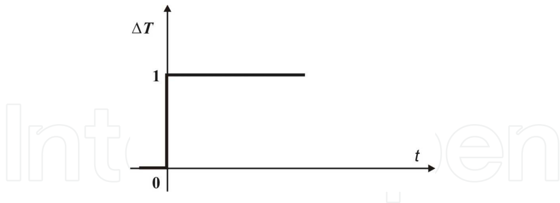
Fig. 4. Temperature step function of the fluid at the tube inlet where:
