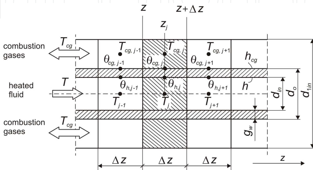
Fig. 1. Analysed control volume of double-pipe heat exchanger
