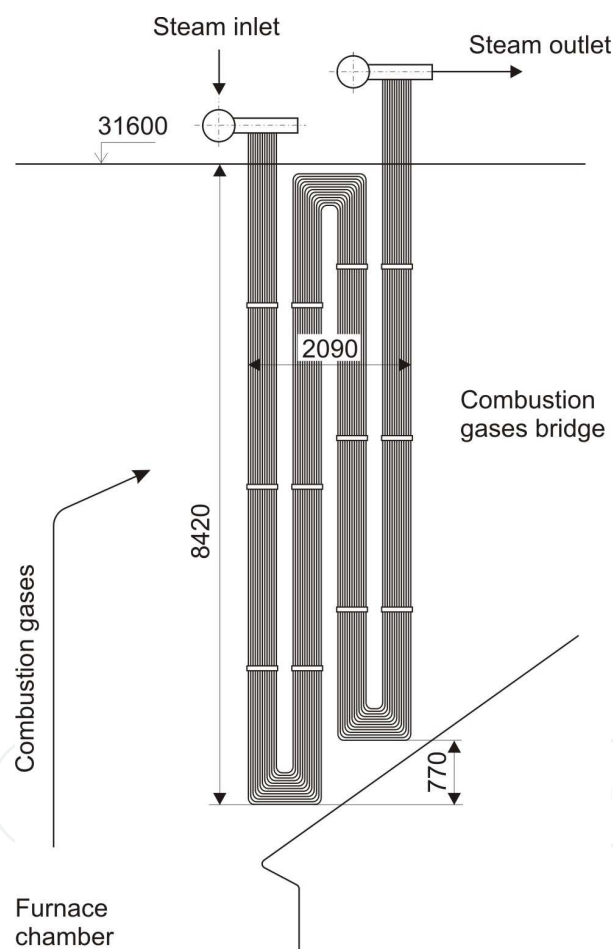
Fig. 8. Location of platen superheater
