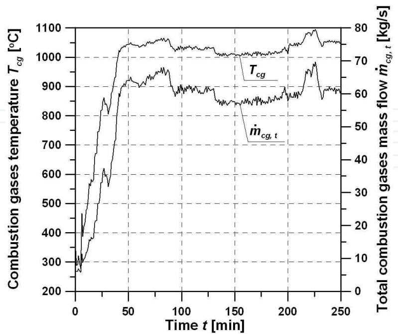
Fig. 10. Histories of the computed combustion gases temperature and total mass flow at the platen superheater inlet (at the furnace chamber outlet)
