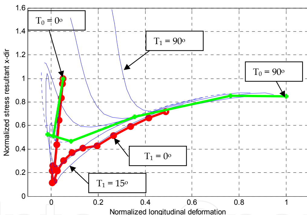
Fig. 11. Normalized longitudinal stress resultant for [0 \pm T_0 | T_1]_{2S}
