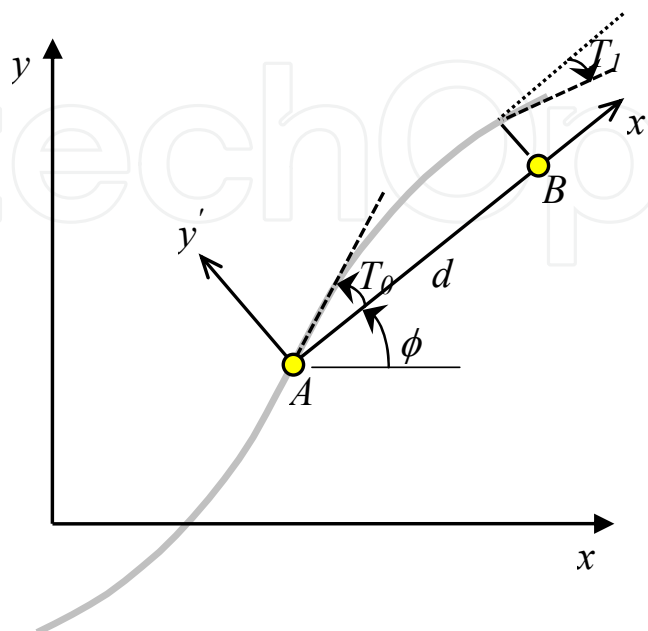
Fig. 1. Reference path definition of a variable layer
