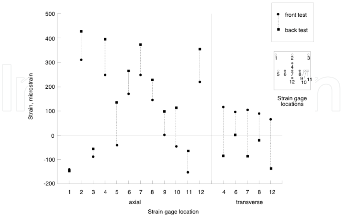
Fig. 17. Maximum strains for panel with overlaps.
