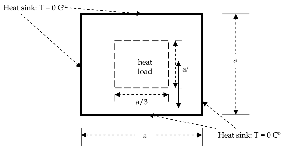
Fig. 4. Square variable stiffness panel under thermal load.
