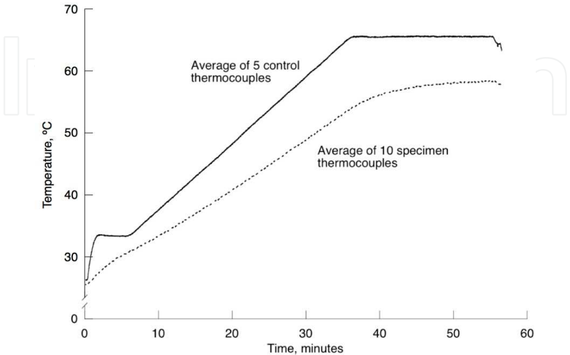
Fig. 14. Temperature profiles for thermal tests.
