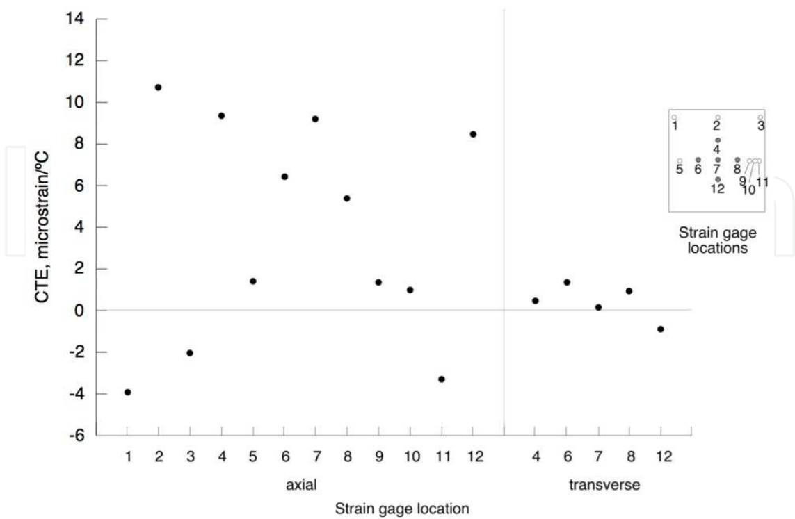
Fig. 18. CTEs for panel with overlaps.
