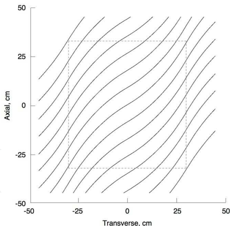
Fig. 13. Variable stiffness panel tow paths.
