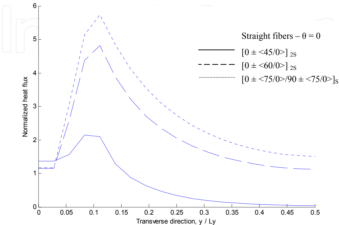
Fig. 10. Heat Flux along transverse direction for one-quarter of plate
