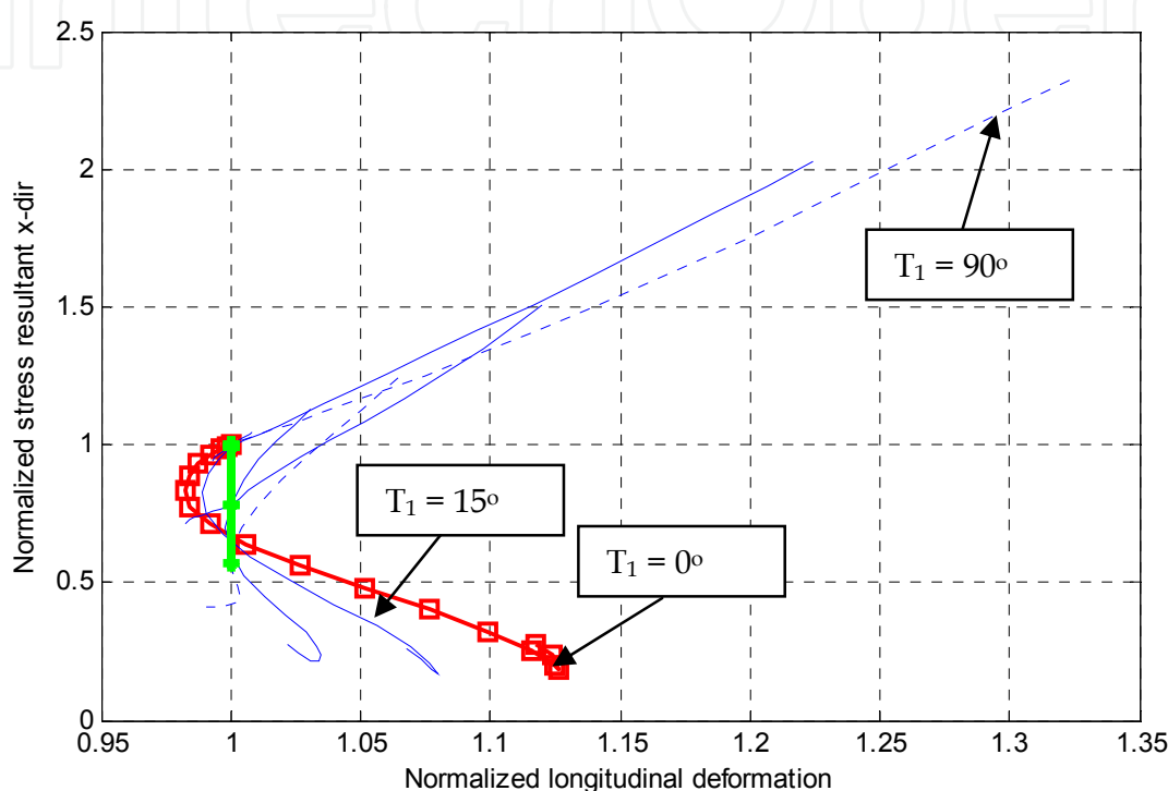
Fig. 12. Normalized longitudinal stress resultant for [0 \pm \langle T_0/T_1 \rangle / 90 \pm \langle T_0/T_1 \rangle]_s
