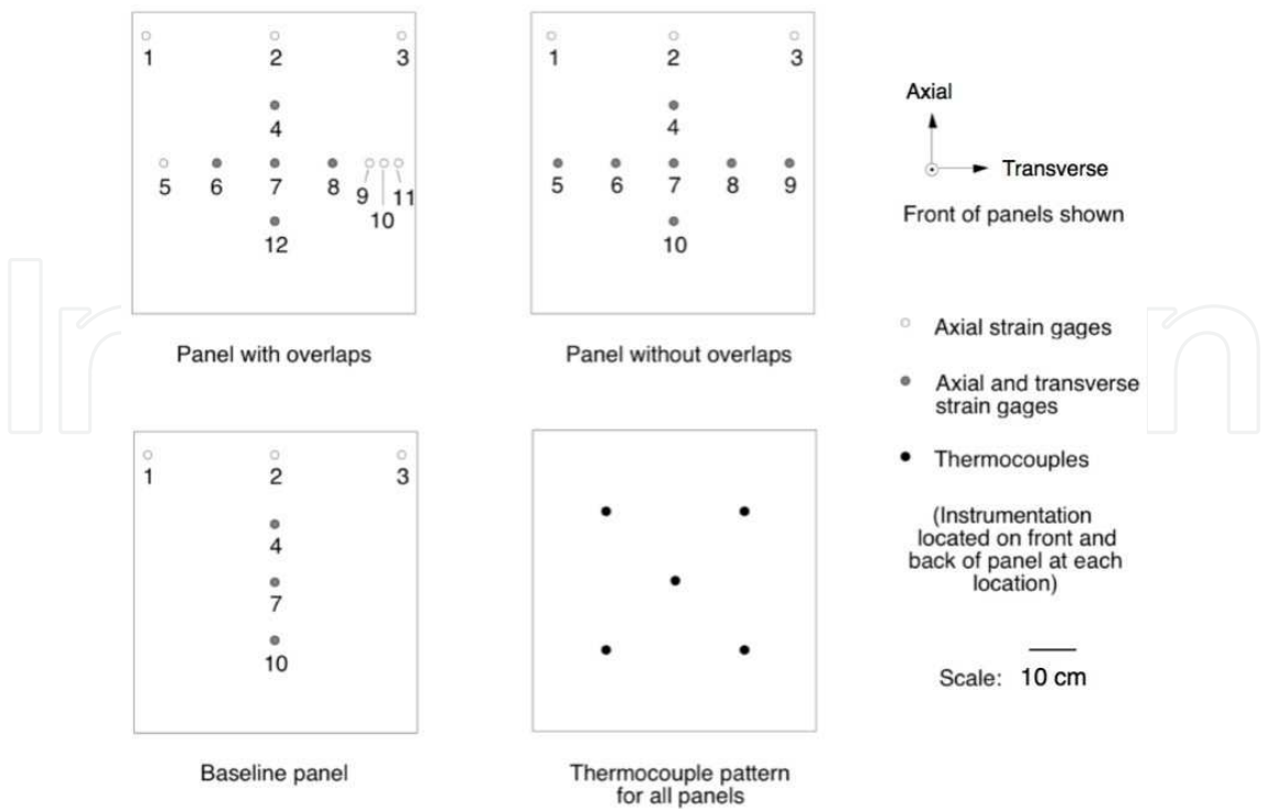
Fig. 15. Composite panel instrumentation.
