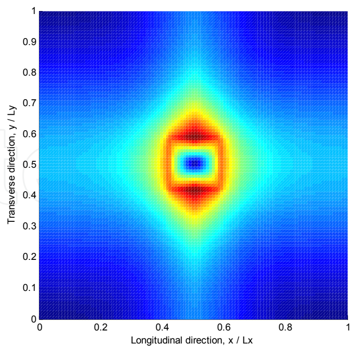
Fig. 8. Heat Flux for [0 \pm 60/0]_{2S} VS laminate.
