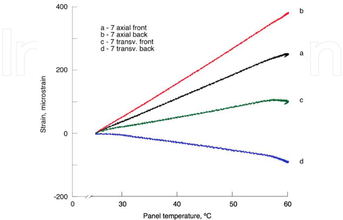
Fig. 16. Strain vs. temperature at center of panel with overlaps.
