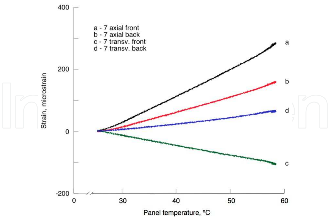
Fig. 19. Strain vs. temperature at center of panel without overlaps.
