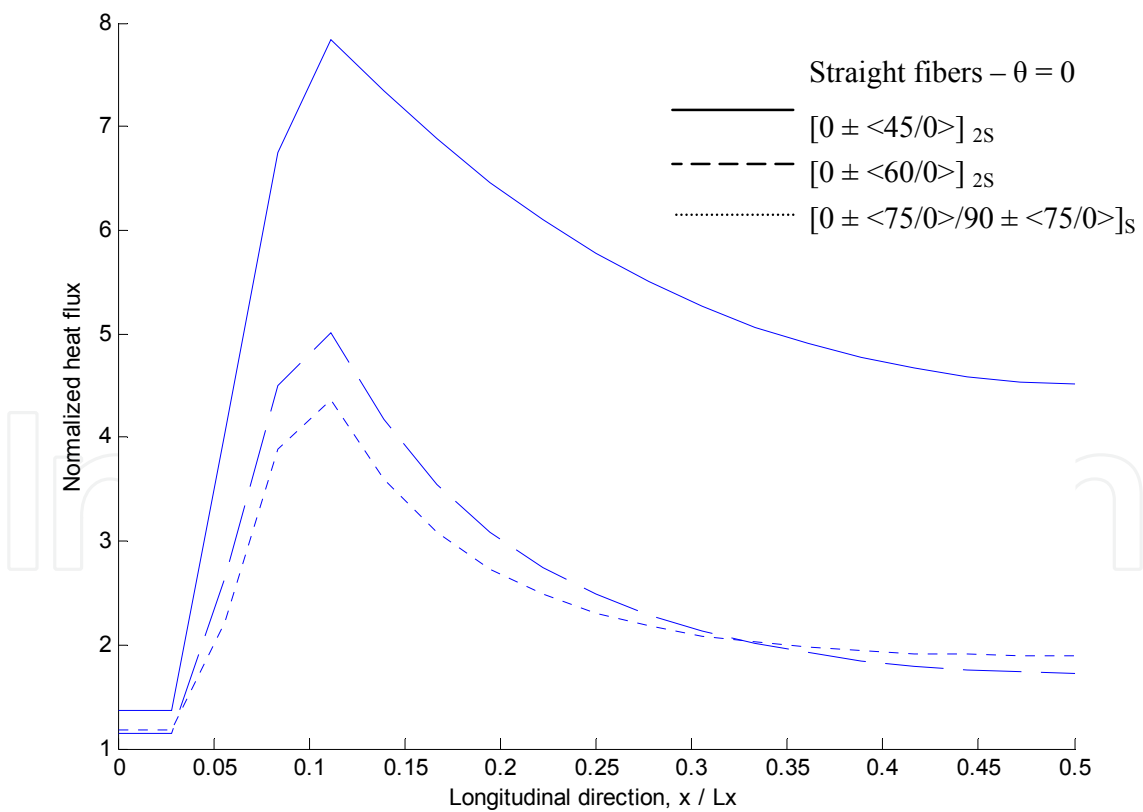
Fig. 9. Heat Flux along longitudinal direction for one-quarter of plate
