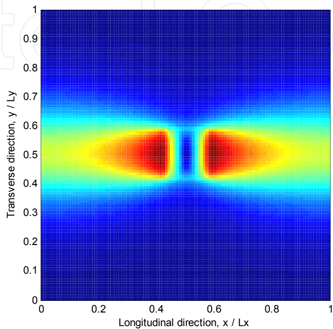
Fig. 6. Heat Flux for 0° straight angle laminate.
