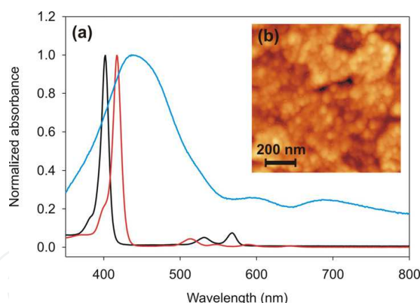
Fig. 15. (a) Normalized UV-visible absorption spectra of ZnOEP in 1,2- \text{C}_2\text{H}_4\text{Cl}_2 (—), of 5,15- \text{H}_2\text{Py}_2\text{Ph}_2\text{P} in 1,2- \text{C}_2\text{H}_4\text{Cl}_2 (—), and of an ITO electrode modified with the copolymer obtained from ZnOEP and 5,15- \text{H}_2\text{Py}_2\text{Ph}_2\text{P} after 25 iterative scans (—). (b) Atomic force micrograph of the same copolymer after washing with water.
