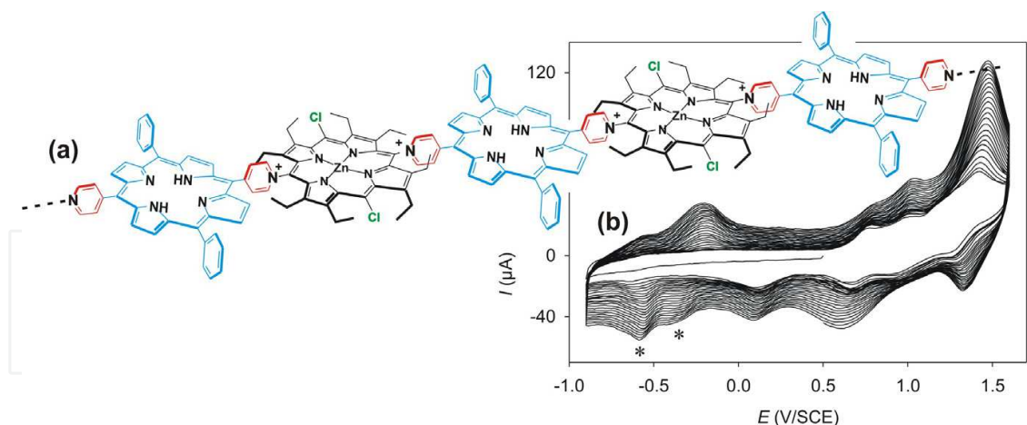
Fig. 14. (a) Scheme of the linear bis-porphyrin copolymer obtained. (b) Cyclic voltammograms recorded during the iterative scans between -0.90 and +1.60 V/SCE of 5,15-ZnOEP( \text{Cl} ) _2 ( 0.25 mM) in the presence of 5,15- \text{H}_2\text{Py}_2\text{Ph}_2\text{P} ( 0.75 mM) in 1,2- \text{C}_2\text{H}_4\text{Cl}_2/\text{CH}_3\text{CN} (4:1) and 0.1 M \text{NBu}_4\text{PF}_6 . Working electrode: ITO; S = 1 cm ^2 ; v = 0.2 V s ^{-1} .
