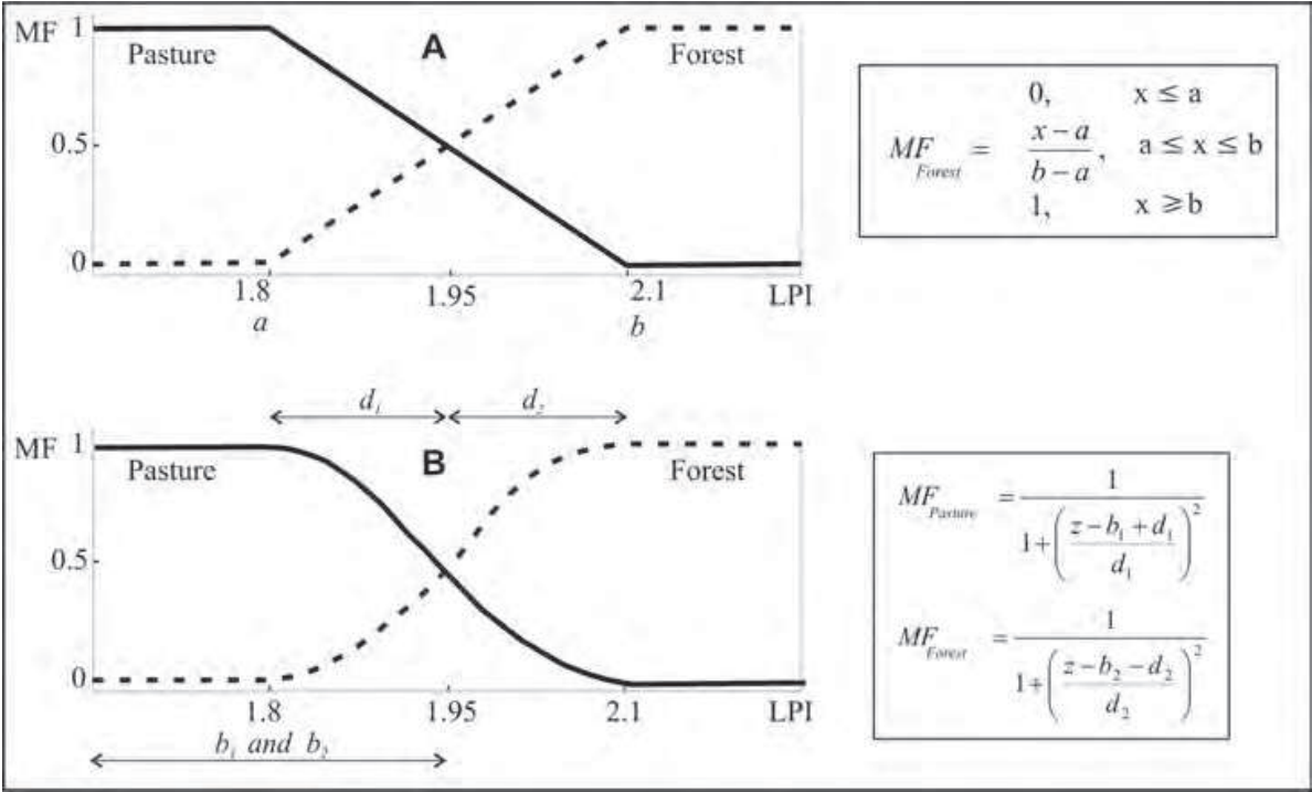
Fig. 4. Membership functions: (A) linear; (B) bell-shaped
