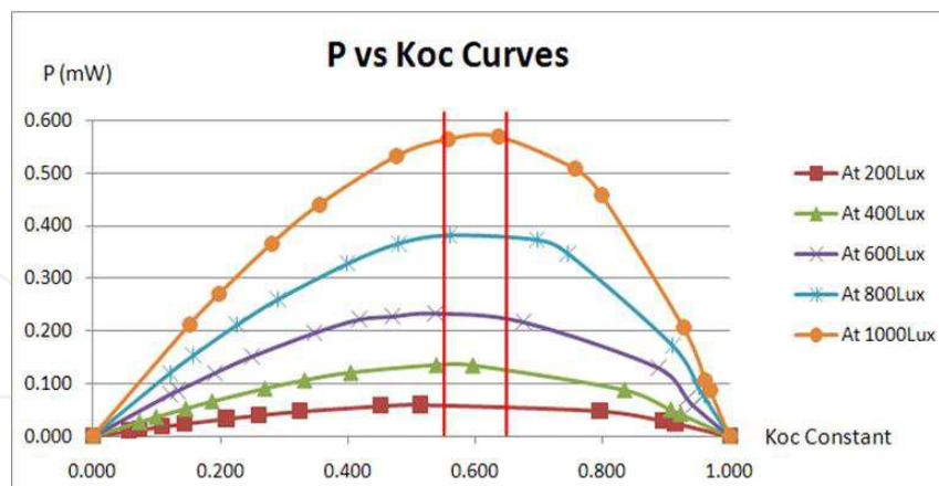
Fig. 8. Graph of Power vs Koc Constants
