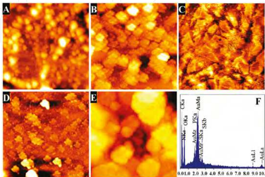
Fig. 10. AFM images of (A) the pristine nanogold bioconjugate (NGBC) and the (B) malathion, (C) parathion, (D) chlorpyrifos, and (E) dimethoate-adsorbed NGBC material. (F) EDXA spectrum of NGBC material after adsorption of organophosphorous pesticide. Langmuir 2009, 25(14), 8192-8199.
