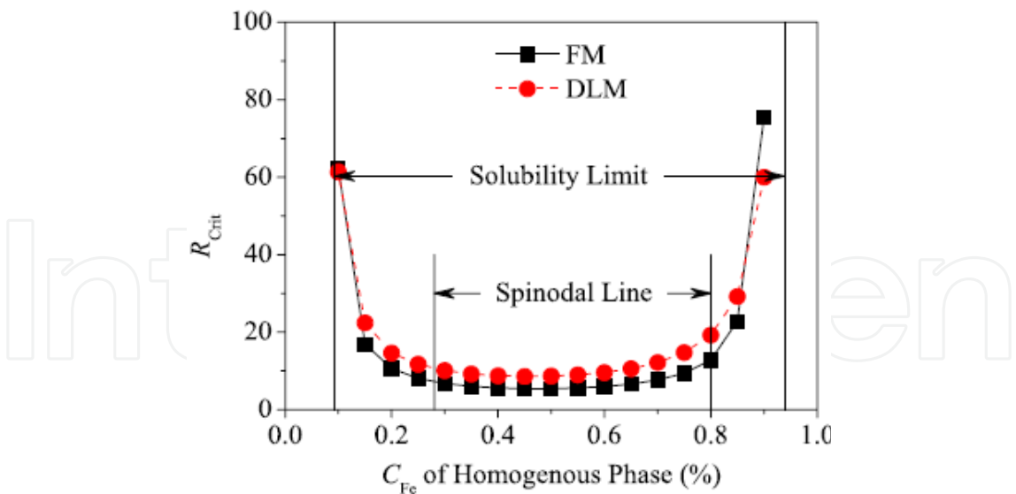
Fig. 7. Critical nucleus size ( R_{crit} in Å) as a function of the composition of the homogenous phase Fe_cCr_{1-c} for ferromagnetic and paramagnetic states. The vertical lines show the experimental spinodal and solubility limits.
