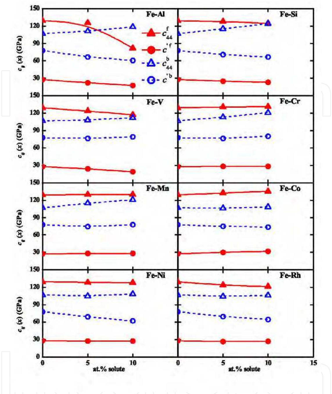
Fig. 2. Single-crystal shear elastic constants c'(x) and c_{44}(x) for paramagnetic fcc (solid symbols connected with solid lines) and ferromagnetic bcc (blue open symbols connected with dashed lines) Fe_{1-x}M_x ( M=Al, Si, V, Cr, Mn, Co, Ni, \text{ and } Rh; 0 \leq x \leq 0.1 ) random alloys. The superscripts f and b denote the fcc and bcc phases, respectively.
