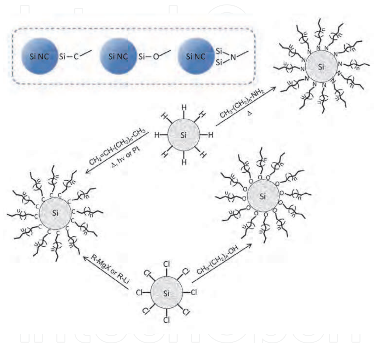
Fig. 16. Representative modification routes for monolayer attachment to the surfaces of hydrogen- and chloride-terminated silicon nanoparticles.
