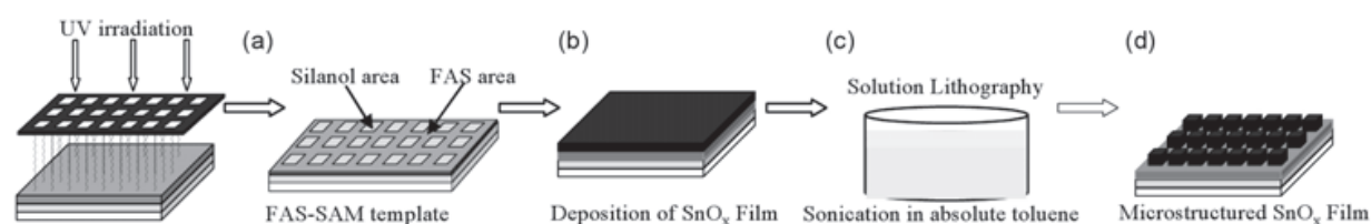
Fig. 6. Schematic illustration showing the microfabrication process of metal oxide film on \text{PI}_{\text{ox}} substrate.
