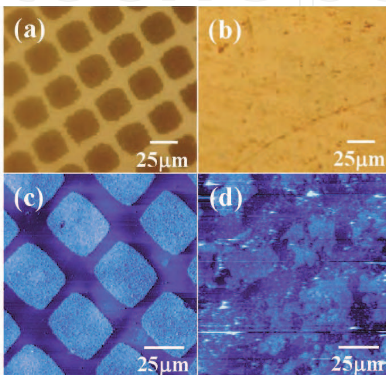
Fig. 7. Optical (a and b) and DFM images (c and d) of tin oxide film microstructured on two different substrates: (a), (c) on FAS/nanolayer/ \text{PI}_{\text{ox}} substrate, while (b), (d) on FAS/ \text{PI}_{\text{ox}} substrate, directly.
