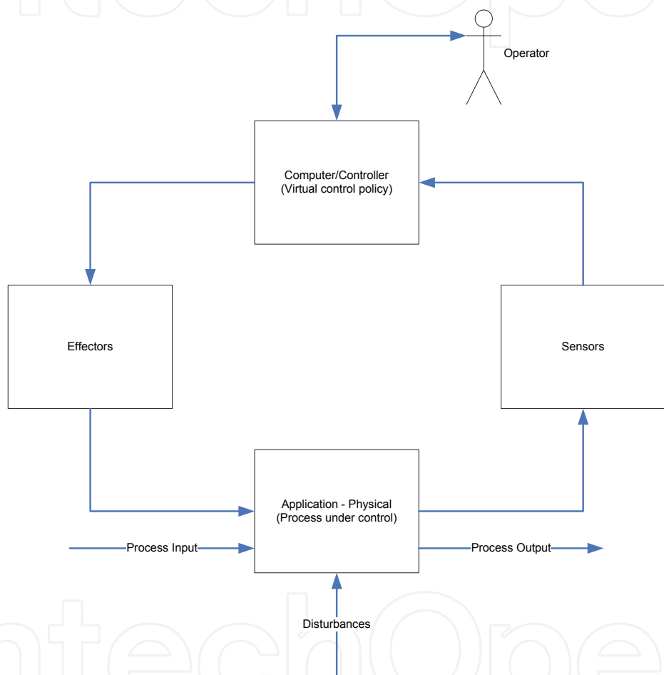
Fig. 2. Traditional Digital Control System Components
