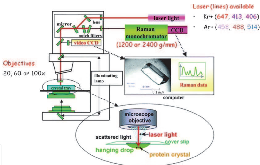
Fig. 1. Scheme of Raman apparatus available at the University of Naples "Ferdinando II" (Dept of Chemistry) to collect spectra from protein single crystals. Adapted after (Carey & Dong, 2004).
