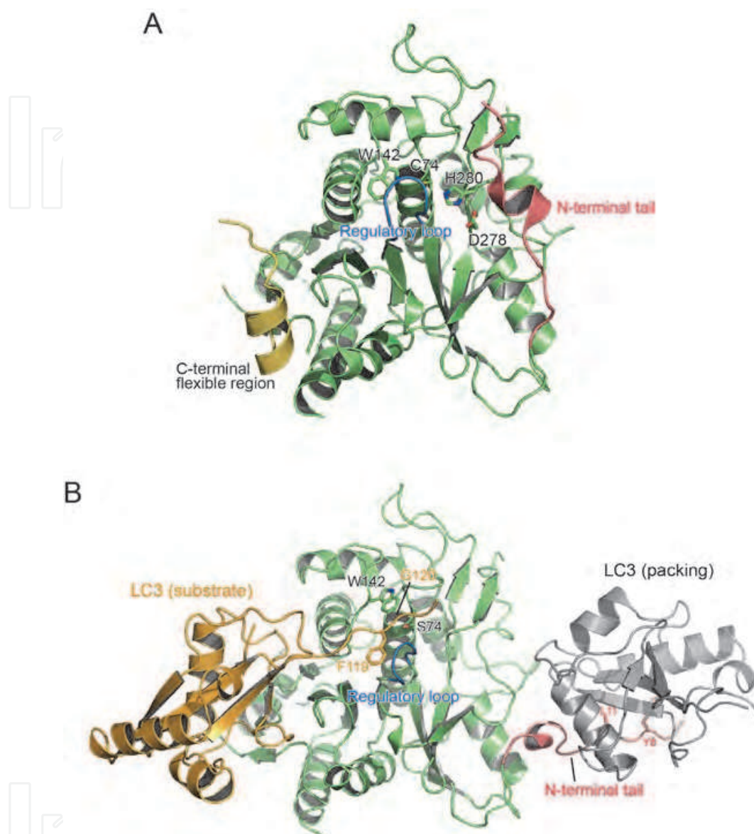
Fig. 5. Structure of HsAtg4B. (A) Free HsAtg4B structure. N-terminal region, regulatory loop as well as C-terminal flexible region are colored salmon pink, blue and yellow, respectively. (B). HsAtg4B-LC3 precursor complex structure. LC3 bound to the catalytic site of HsAtg4B is colored light orange, while LC3 bound to the N-terminal tail of HsAtg4B is colored gray. The other coloring is as in (A).
