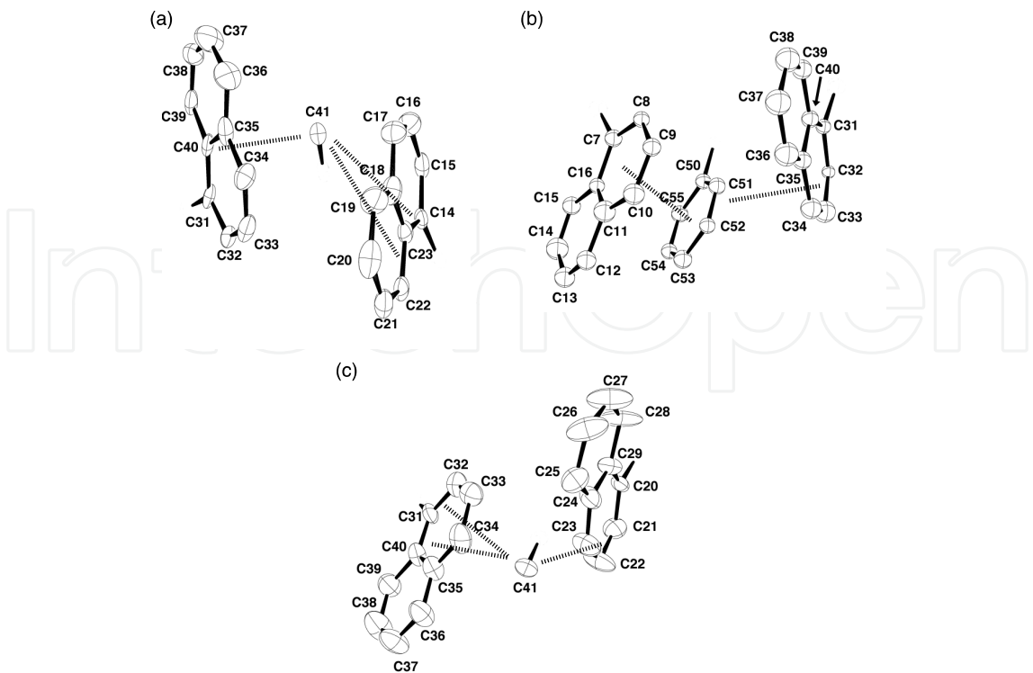
Fig. 5. Intramolecular CH/ \pi and \pi - \pi interactions of (a) 5 , (b) 6 , and (c) 7 Me .
