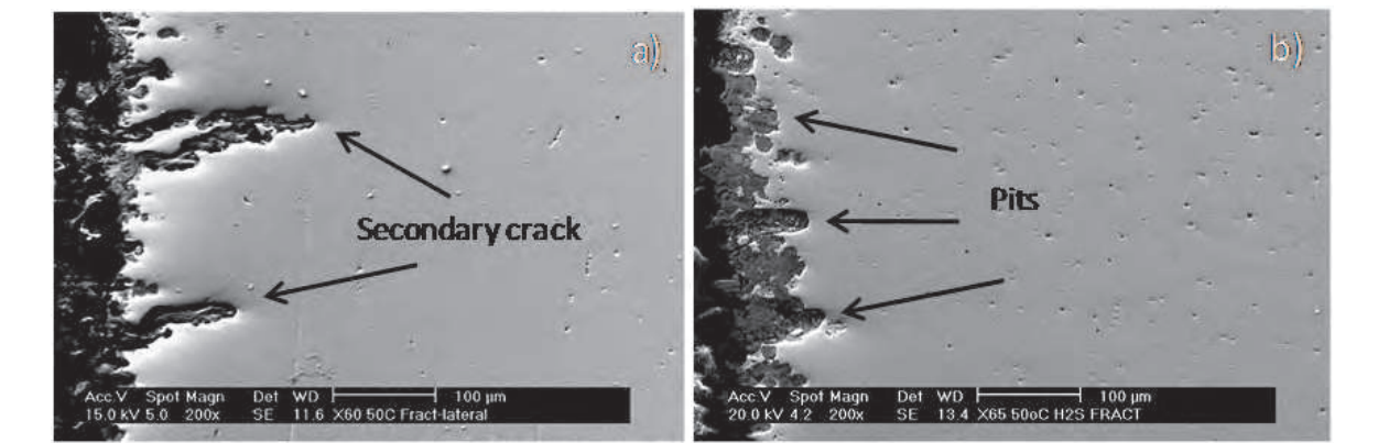
Fig. 15. Cross-sections of weldments tested in the NACE solution saturated with H 2 S. (a)X60 steel at 50°C, (b)X65 steel at 50°C.
