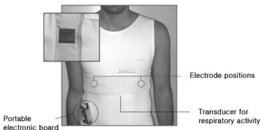
Fig. 4. The MagIC system
