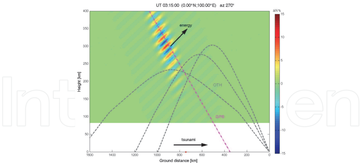
Fig. 6. Vertical cross section of the modeled tsunami-related electron density perturbation and ray-paths computed using a 10 MHz OTH radar signal at 19°, 30° and 35° elevation (dashed gray lines). Dash-dotted purple line indicates a possible geometry of a nearby GPS station for a satellite at 25° elevation. Arrows indicate the tsunami and IGW energy directions of propagation. Note that the vertical scale has been exaggerated. Figure after Coisson et al. (2011).
