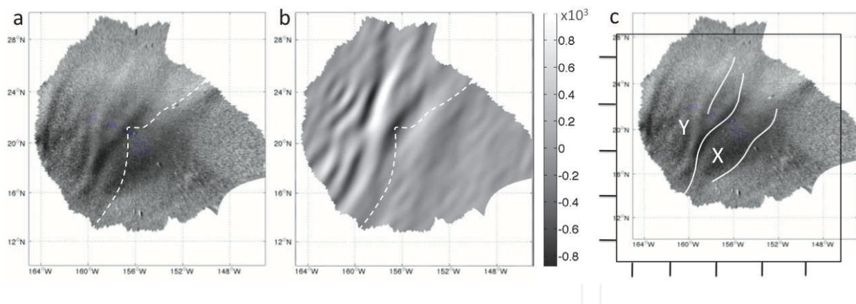
Fig. 10. a) IGW imaged by the 630.0-nm ground-based airglow camera located on the Haleakala Volcano on Maui, Hawaii, at 13:20 UT. b) normalized vertical velocity of the modeled IGW ( (\text{kg}/\text{m}^3)^{\frac{1}{2}} \text{m/s} ). The Y structure as well as the longer wavelength anticipating the Y (X) are present in both, airglow data and AGW synthetics. Those structures are observed between 12:12 to 13:32. The white dotted line in a and b shows the tsunami wavefront line at 13:20 UT. c) graphical estimation of the shift induced by the wind between model and data: the grid and the white lines are estimated on b, then shifted on a to fit with the position of Y and X. The estimated shift of 2^\circ is coherent with previous observations Occhipinti et al. (2006). Figure after Occhipinti et al. (2011a).
