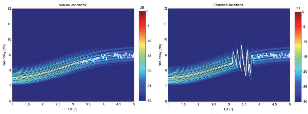
Fig. 7. Synthetic OTH radar record from 01:00 to 0605:00 UT at 270° azimuth 30° elevation during tsunami related IGW propagation showed in Fig. 6. Left: unperturbed ionosphere. Right: ionosphere with IGW perturbation. White points indicate the maximum signal strength at each UT. Figure after Coisson et al. (2011).
