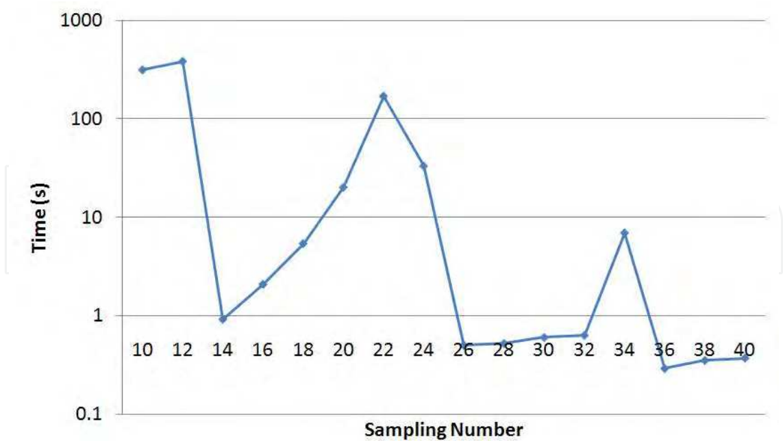
Fig. 15. The effect of sample size on computation time.
