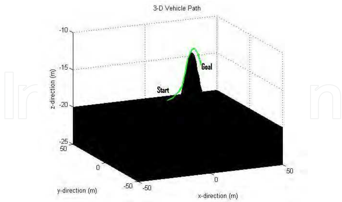
Fig. 10. The AUV kinematic model steep hill scenario.
