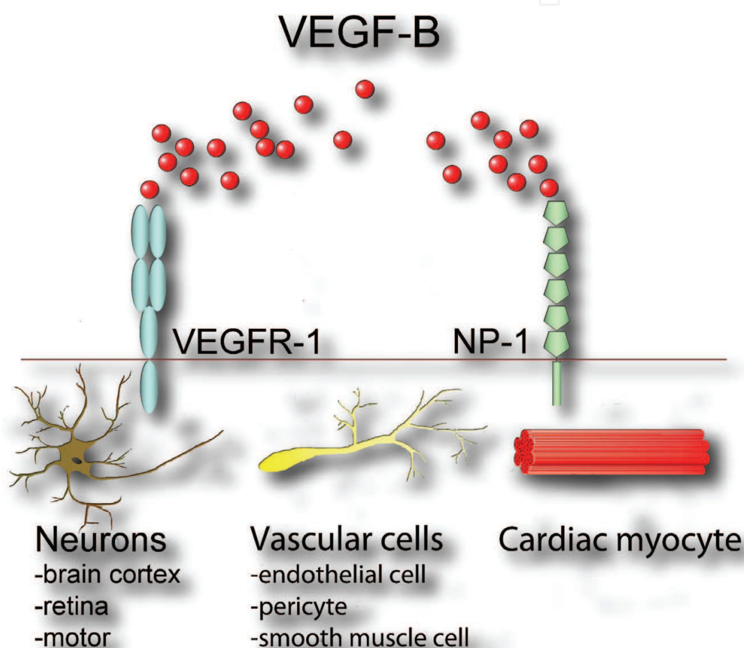
Fig. 1. Pleiotropic protective/survival effect of VEGF-B on multiple cell types. Both in vitro data derived from cultured neurons and in vivo work using different types of animal models have shown that VEGF-B is a critical protective/survival factor for different types of neurons, including cortical, retinal, and spinal cord motor neurons. In addition, VEGF-B is also a potent protective/survival factor for different types of vascular cells, including vascular endothelial cells, smooth muscle cells and pericytes. Moreover, VEGF-B has also been reported to be a protective factor for cardiac myocytes
