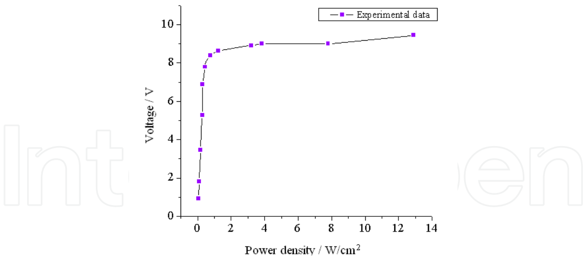
Fig. 19. The response curve of PC-10.6 detector irradiated by pulse laser
