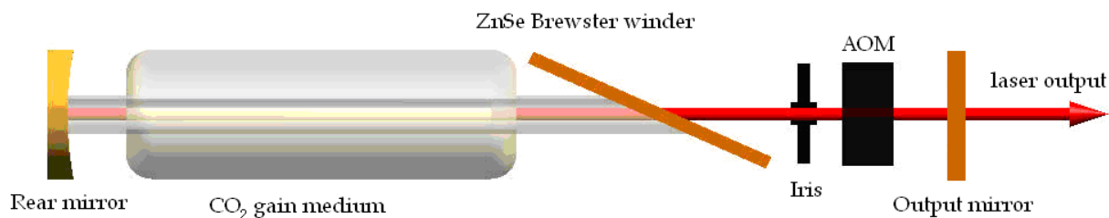
Fig. 2. Schematic diagram of acousto-optically Q-switch CO 2 laser
