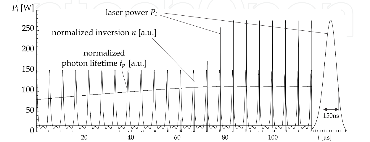
Fig. 10. Simulation results of Nd:YAG-rod laser based on Fig. 8 and Eq. 6.
