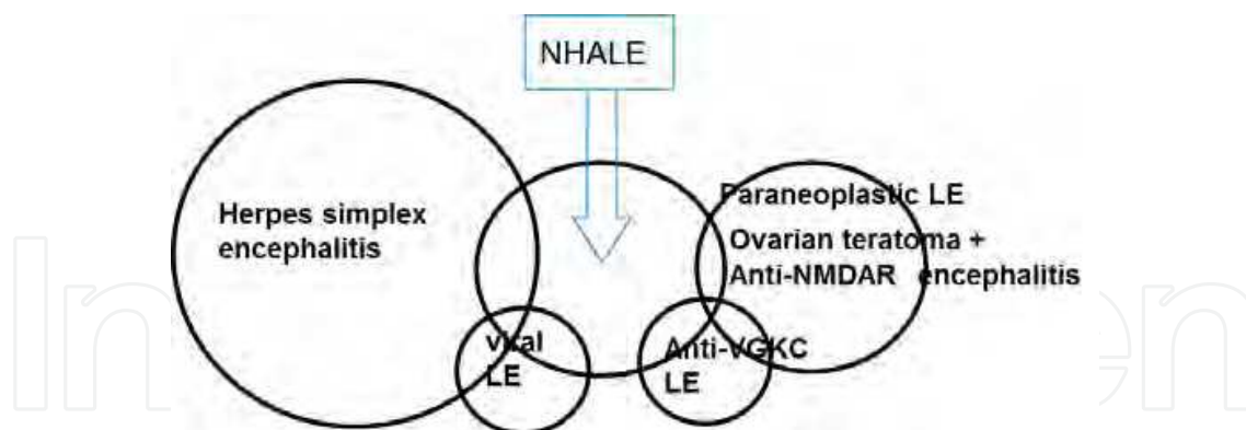
Fig. 1. Possible relationships of NHALE and related disorders.
