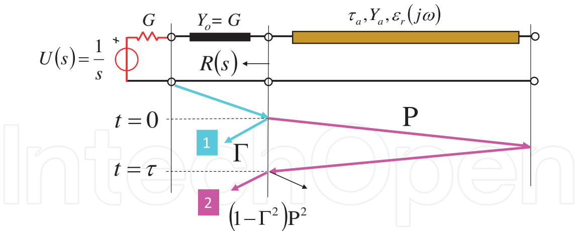
Fig. 7. Simplified transmission line model of the TDR measurement system and bouncing diagram. First contribution ( \bar{\Gamma} : the signal reflected at the input port of the probe (partial reflection coefficient)); second contribution (1 - \bar{\Gamma}^2(S)) \bar{P}^2(S) : the signal transmitted and traveling forward and backward along the probe.
