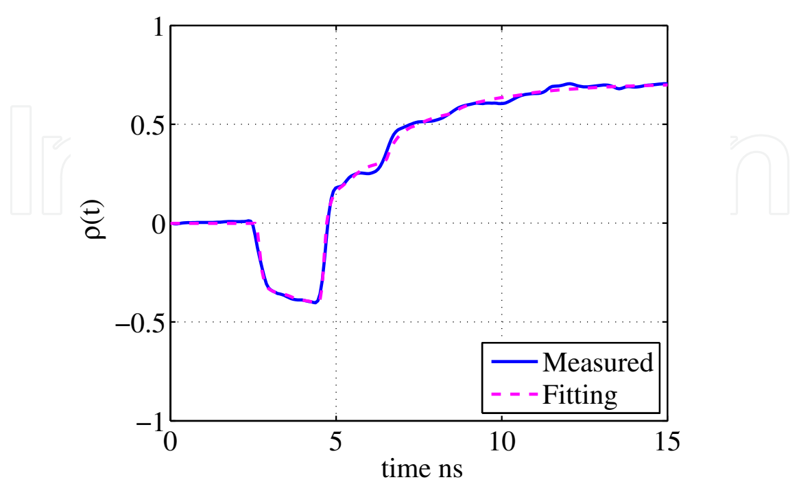
Fig. 17. Measured TDR response for a sand sample with 25% water content (solid line) and the best fit response of the accurate model (dashed line). Permittivity parameters: \epsilon_s = 12. , \epsilon_\infty = 8.4 , f_{rel} = 1.38 GHz and \sigma_s = 0.007 S/m.
