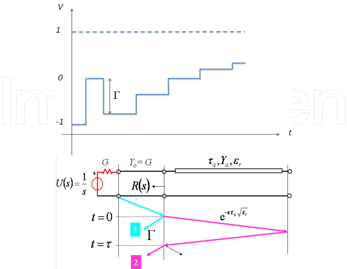
Fig. 2. TDR response and bouncing diagram of the TDR system.
