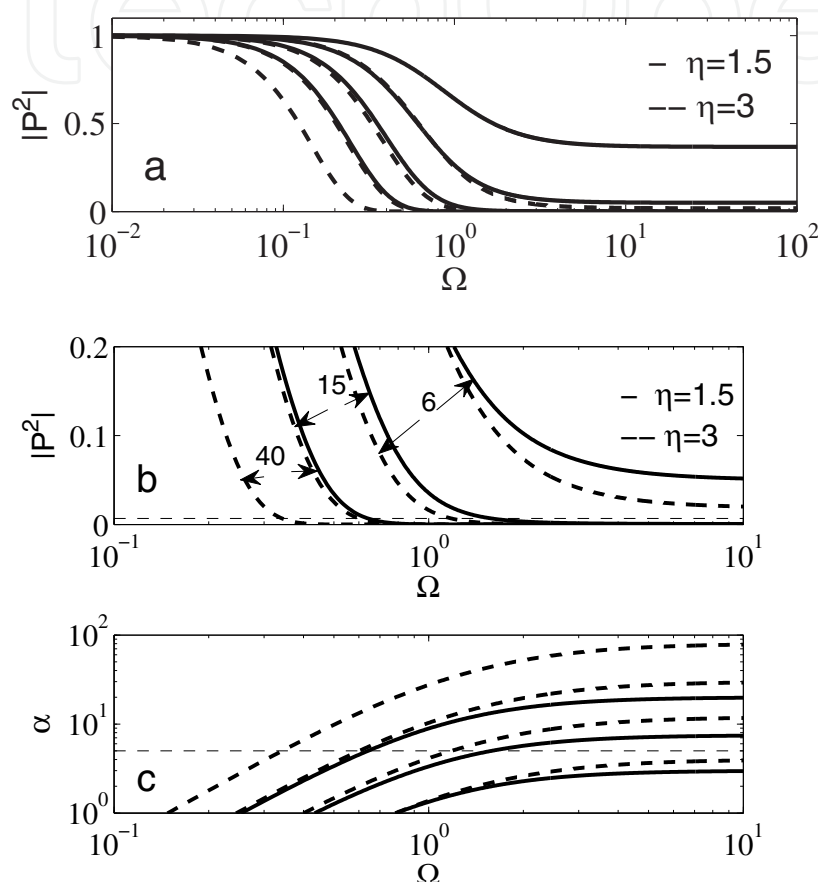
Fig. 8. Magnitude of the propagation factor (a and b) and attenuation constant (c) versus normalized angular frequency for T = 6, 15, 40 and \eta = 1.5, 3 . Panel b is a close-up view of panel a. The dashed horizontal lines of panel b and c indicate the threshold level |\bar{P}^2| = \exp(-5) and \zeta = 5 , respectively.
