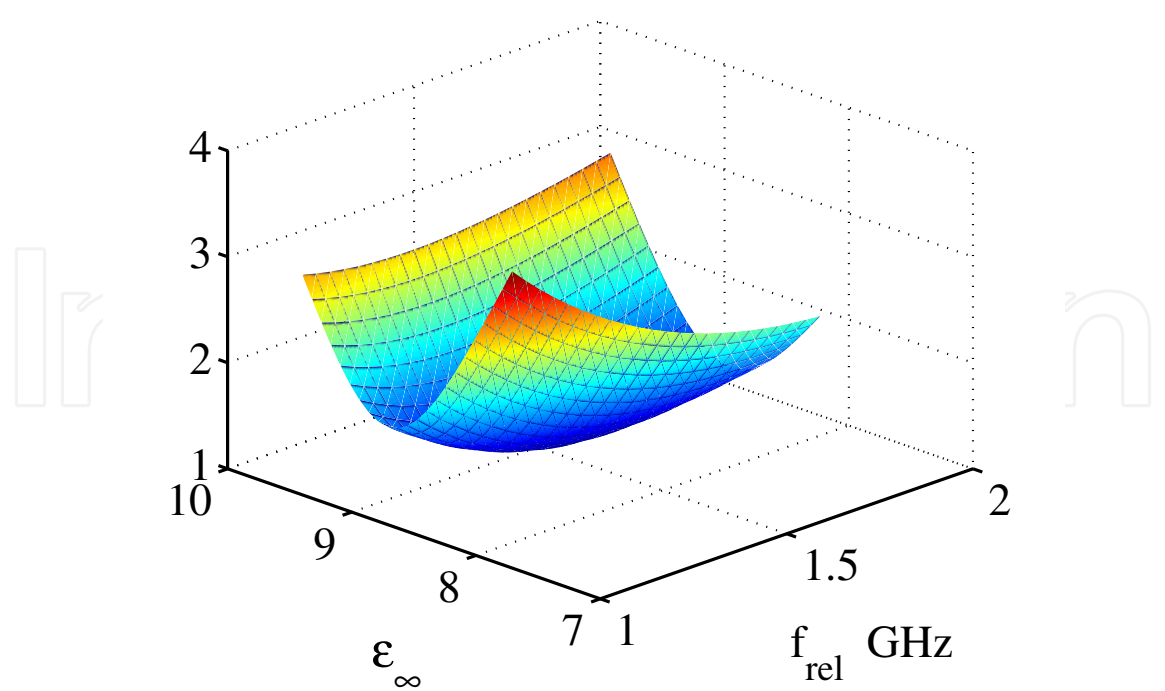
Fig. 18. Error surface in the (\epsilon_\infty, f_{rel}) plane for a sand sample with 25% water content.
