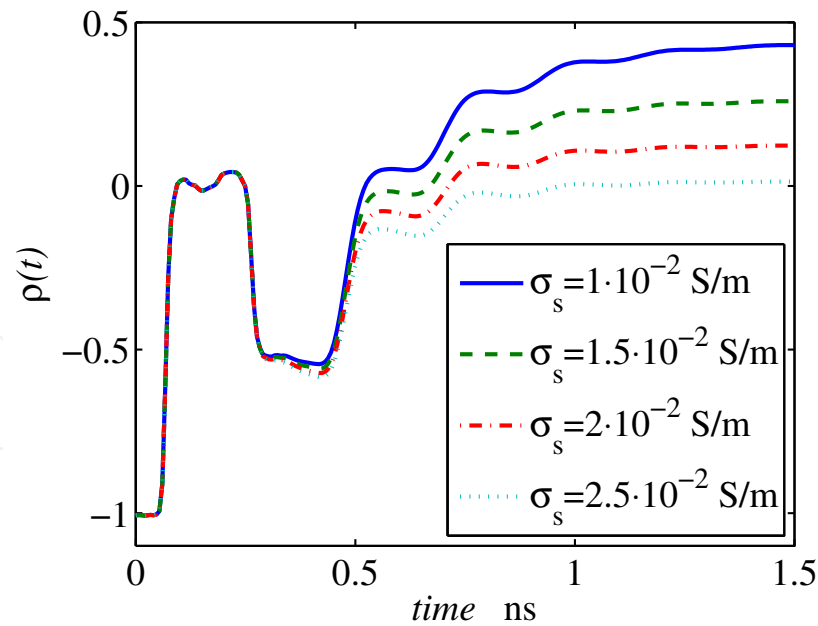
Fig. 13. Model response for different values of \sigma_s(1 \cdot 10^{-2}, 1.5 \cdot 10^{-2}, 2 \cdot 10^{-2}, 2.5 \cdot 10^{-2}) S/m. Other parameter values are \omega_{rel} = 20 \cdot 10^9 ; \epsilon_s = 10 ; \epsilon_{\infty} = 3 .
