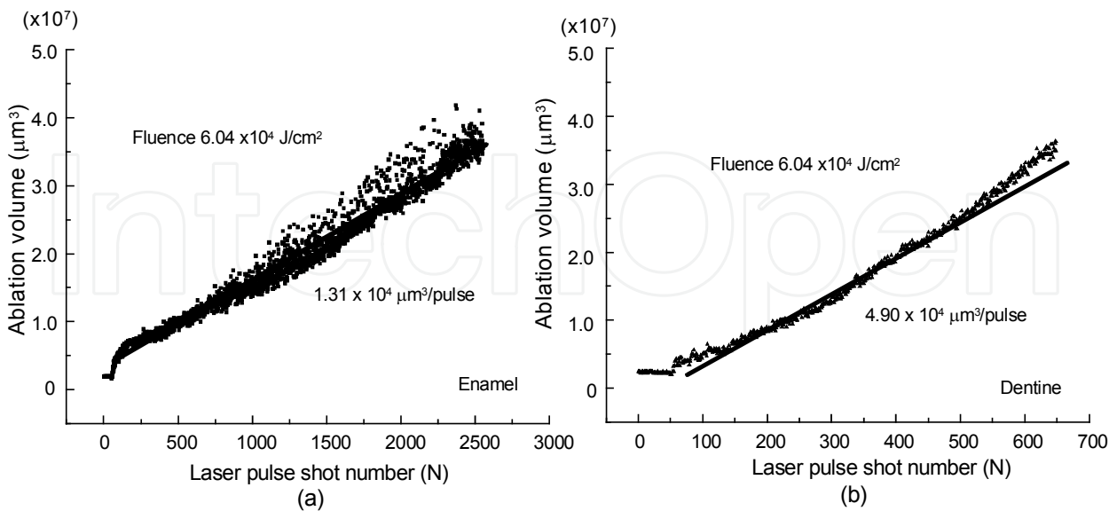
Fig. 8. Measured ablation volume versus laser shot number. (a) Enamel, (b) Dentine.
