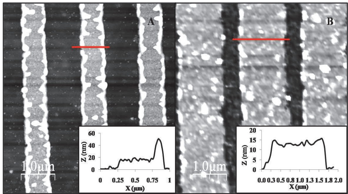
Fig. 5. AFM images of lift-off patterning procedure including line scan along the red line. A) 15 nm of Ag on top of a coverage grating formed via a 50ML Xe on Ti/SiO 2 /Si surface. First and second pulse power were both of 10 MW/cm 2 . B) 12 nm of Ag on top of grating produced with 70ML Xe on top of Ti/SiO 2 /Si surface. Both the first and second pulses were at 14 MW/cm 2 .
