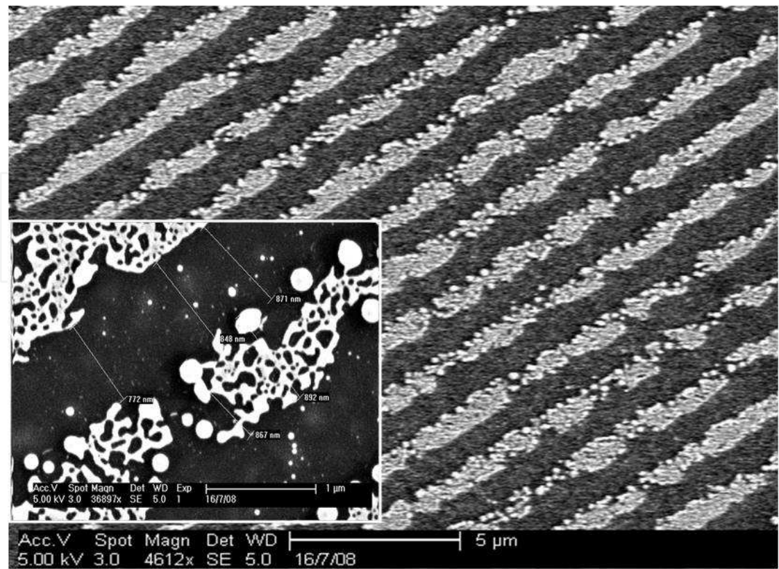
Fig. 4. SEM image of lift- off patterning of 18 nm Au on top of SiO 2 /Si surface. The power of the first and second laser pulses was 12 and 9MW/cm 2 , respectively. Inset depicts the corrugated (and fragmented) texture of the resulting metal wires.
