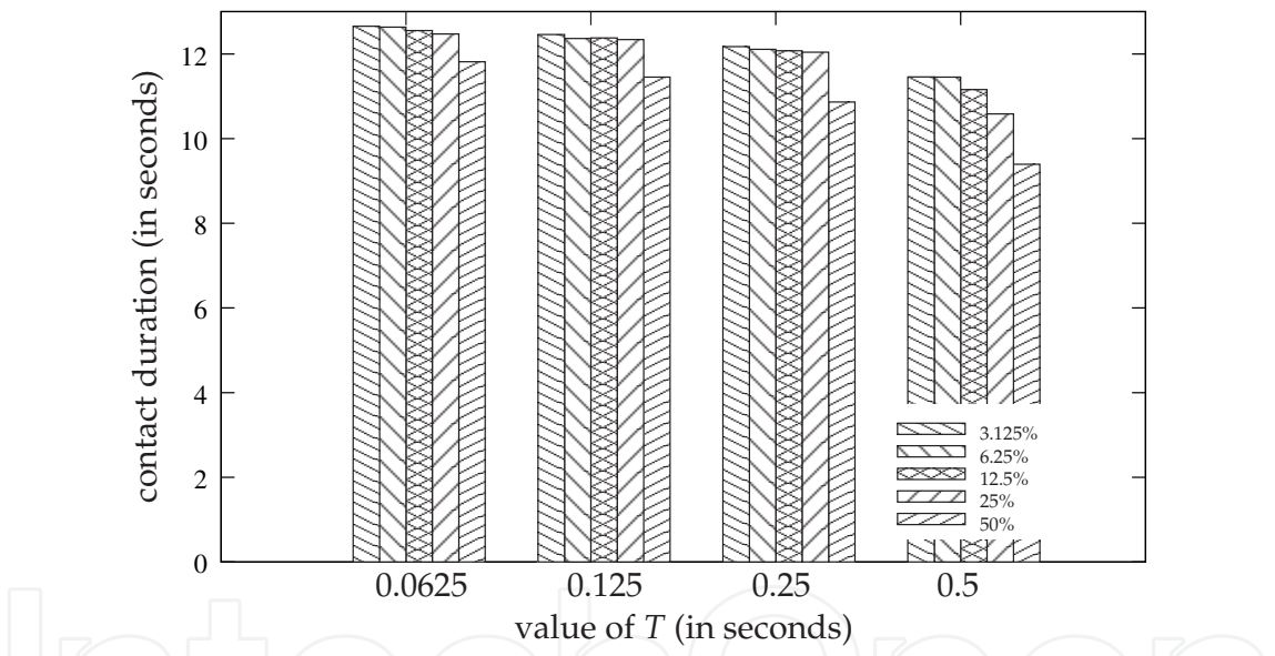
Fig. 8. The neighbor discovery delay is greatly impacted by the duration of the inactivity period.
