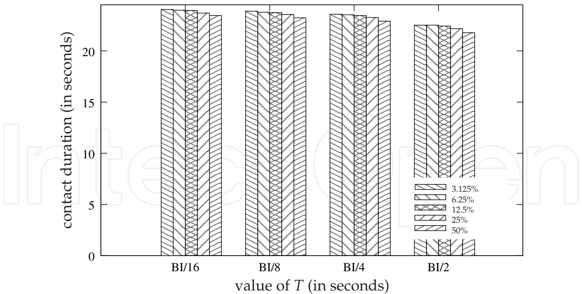
Fig. 14. The contact duration between a mobile and a fixed-relay depends mostly on the GW-ADV periodicity.
