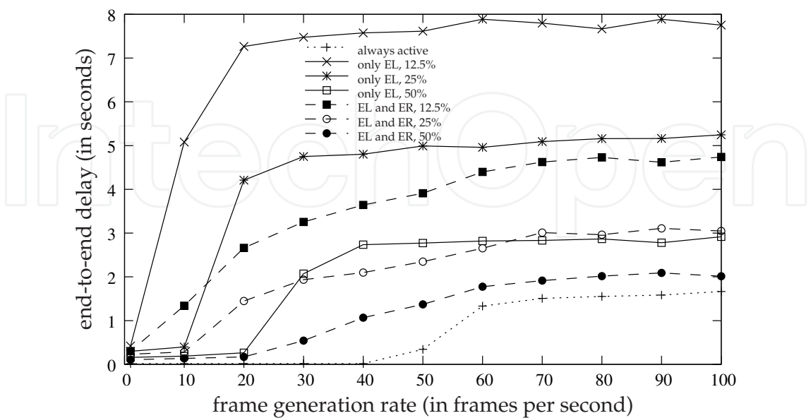
Fig. 5. The presence of ER nodes significantly reduce the end-to-end delay, for all duty cycles.
