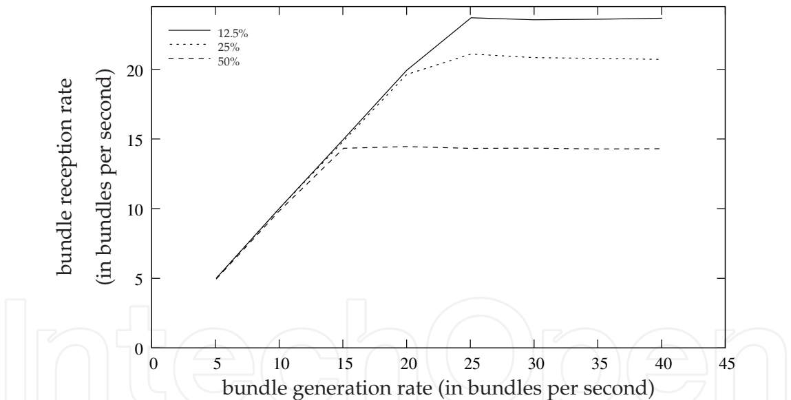
Fig. 15. The bundle reception rate increases when the duty cycle on the robot-specific channel decreases.
