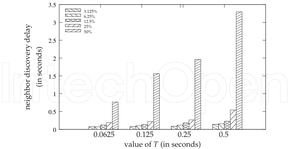
Fig. 7. The neighbor discovery delay is greatly impacted by the duration of the inactivity period.
