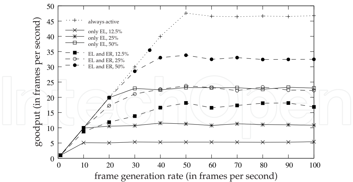
Fig. 4. The presence of ER nodes significantly improves the performance of the network, for all duty cycles.
