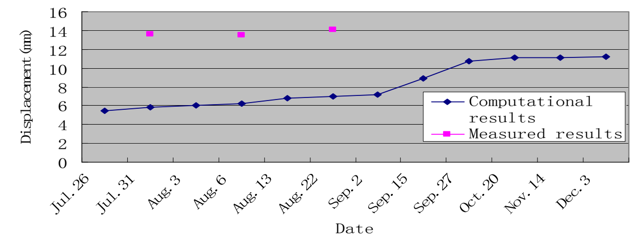
Fig. 6. Graph of the relative displacement change at the arch springing (point F)
