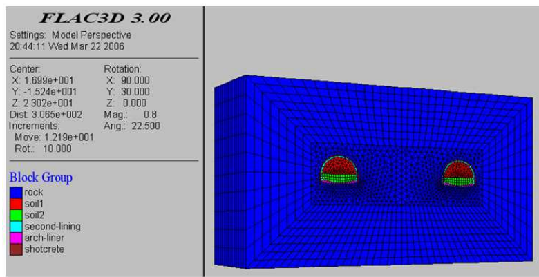
Fig. 2. Numerical computation model
