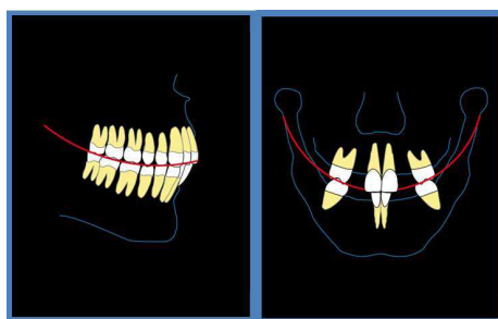
Fig. 4. The curve of Spee and of Wilson
