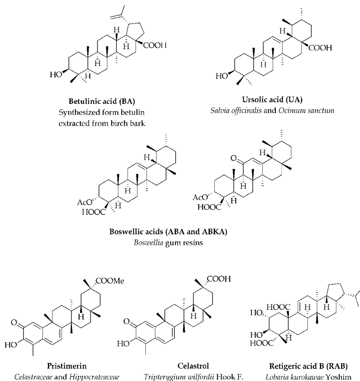
Fig. 7. Pentacyclic triterpenoids
