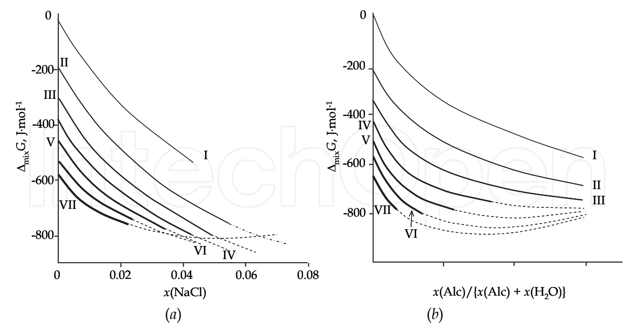
Fig. 5. The isothermal (298.15 K) sections of Gibbs energy surface of solutions of H 2 O- iso -C 3 H 7 OH-NaCl with constant (a) the ratio of water and alcohol; (b) the weight fraction of alcohol in solvent. The numbers correspond to solutions with the weight fraction of alcohol in solvent is: (I) 0, (II) 10.0, (III) 20.0, (IV) 30.0, (V) 40.0, (VI) 49.9, (VII) 58.5 wt. % (a); and with mole fraction of sodium chloride equal to: (I) 0, (II) 0.01, (III) 0.02, (IV) 0.03, (V) 0.04, (VI) 0.05, (VI) 0.06 (b). Dashed lines indicate the extrapolated values of the \Delta_{\text{mix}}G function outside the range of experimental research. The line width increases with the increasing of (a) the weight fraction of alcohol in solvent; (b) the mole fraction of NaCl.
