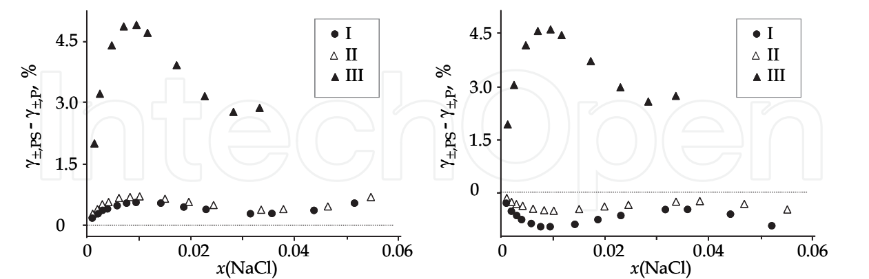
Fig. 4. The difference between Pitzer-Simonson and Pitzer model calculations at 288.15 K (a) and 298.15 K (b). A number I, II and III corresponds to various composition of solvent: 9.99, 19.98 and 39.96 w.%, respectively.
