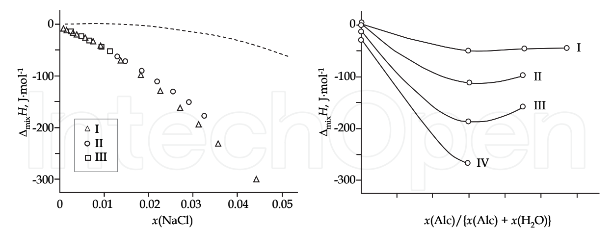
Fig. 6. Isothermal sections of the surface of the enthalpy of mixing of the NaCl-H 2 O- iso -C 4 H 9 OH solution at 298.15 K along the sections with constant water-to-alcohol ratios (a); the weight fraction of the alcohol in the solvent ( w_{\text{Alc}} ) is (I) - 3.0; (II) - 4.5; (III) - 5.66 wt. %, dashed line - without alcohol; (b) along the sections with constant mole fractions of sodium chloride; x_{\text{NaCl}} is (I) - 0.01; (II) - 0.02; (III) - 0.03; (IV) - 0.04. The points in each section at (b) are connected by a solid line.
