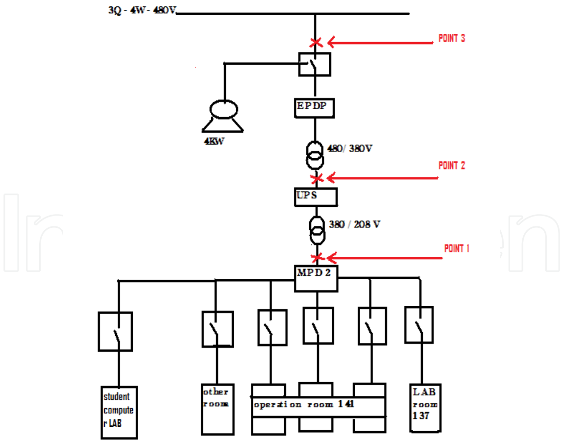
Fig. 4. Building 14 Single Line Diagram and Points of Measurements and switch boards
