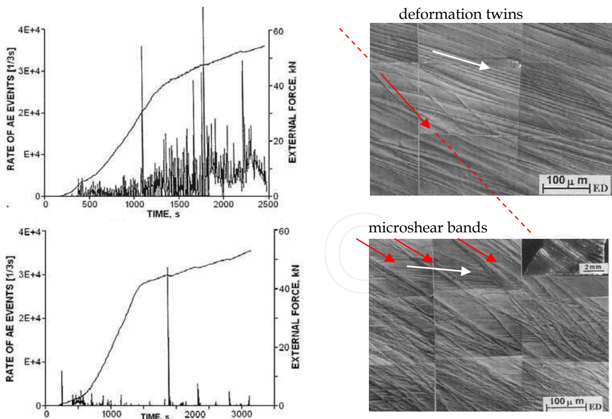
Fig. 16. Courses of AE and external force and corresponding microstructures of Cu single crystals of orientation \{112\}\langle 111 \rangle channel-die compressed at T=77K : (a) – reduction \varepsilon \approx 41\% and (b) – reduction \varepsilon \approx 53.4\%
