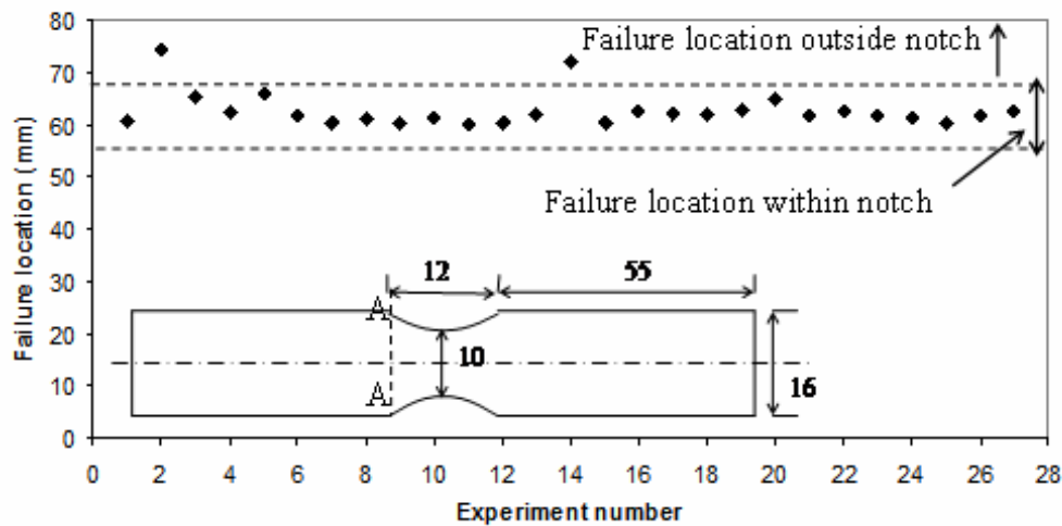
Fig. 13. Failure location in aluminium TWB (Abhishek et al., 2011)
