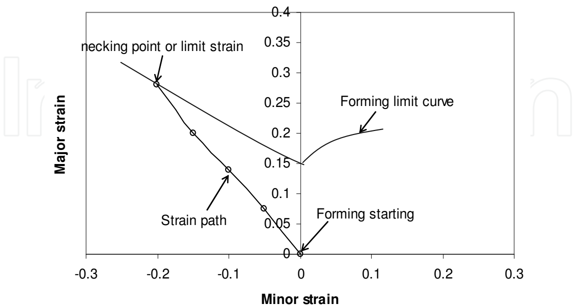
Fig. 11. Schematic representation of strain path with forming limit curve
