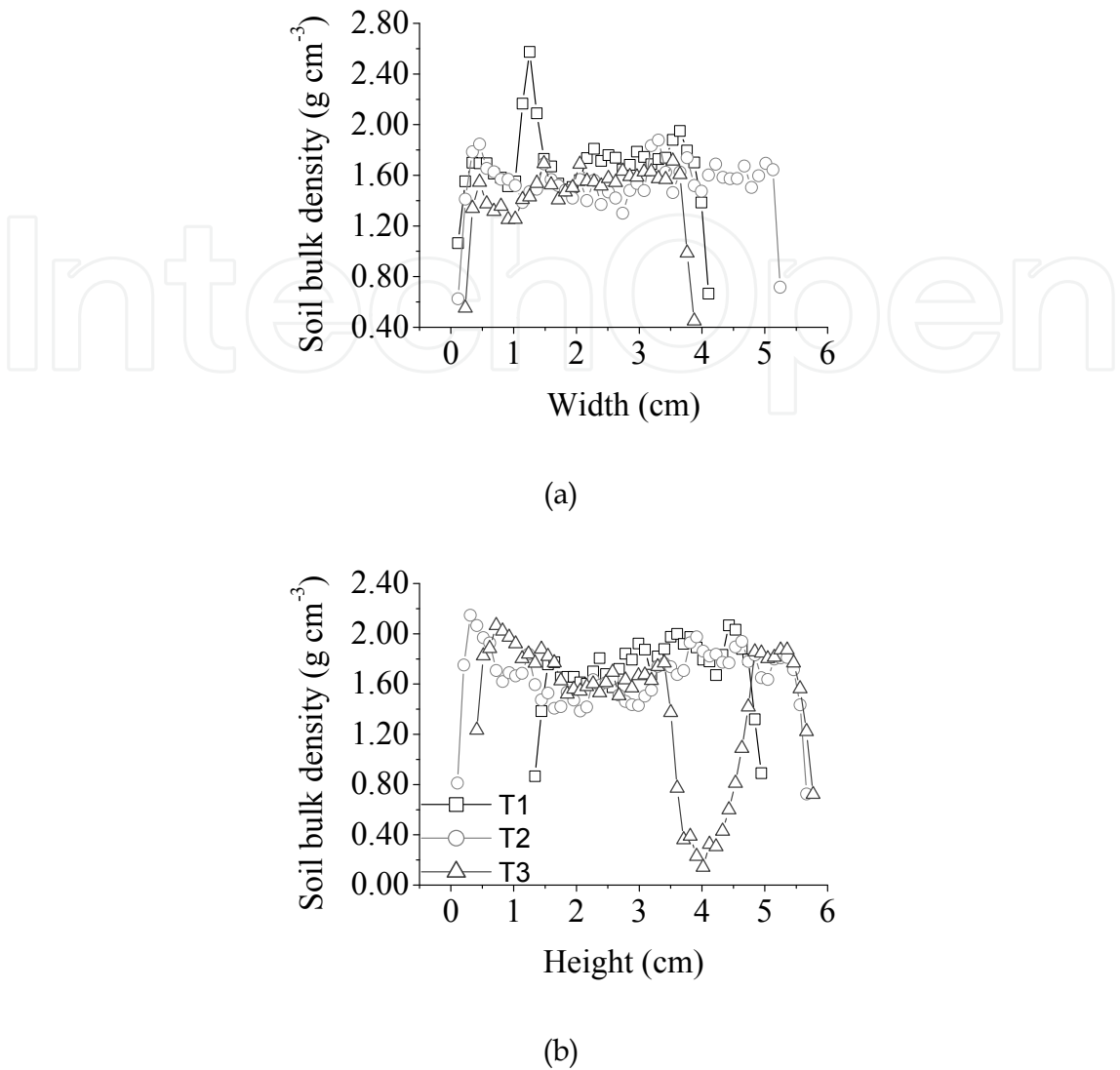
Fig. 5. Soil bulk density ( \rho_s ) values along linear transects (T) inside the soil clods. (a) Analysis along soil width and (b) analysis along soil height.
