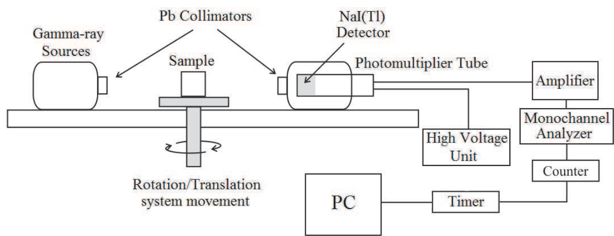
Fig. 2. Schematic diagram of a first generation CT scanner. Adapted from Pires et al. (2011c). The radioactive sources used in the study were 241 Am (59.54 keV) and 137 Cs (661.6 keV), protected by a lead block. A NaI(Tl) scintillation crystal (7.62 x 7.62 cm) coupled to a photomultiplier tube was used to detect the monoenergetic photons passing through cylindrical lead collimators placed either in front of the source as the detector (Figure 3). The gamma detector is also protected by a lead block to minimize background radiation detection. The acquired data were stored in a PC and CT images were obtained using the reconstruction algorithm Microvis (2000). The angular and linear steps were chosen as: 2.25° and 0.11 to 0.15 cm, respectively.
