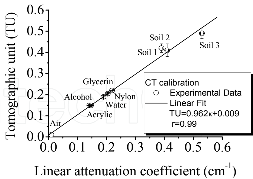
Fig. 1. Computed tomography (CT) calibration curve for 241 Am gamma-ray radiation. Error bars represent the standard deviation of the measurements. Soil 1, 2 and 3 are sand, clay loam and clay sieved soils.
