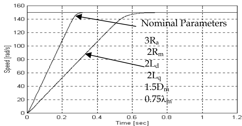
Fig. 5. Robustness test.
