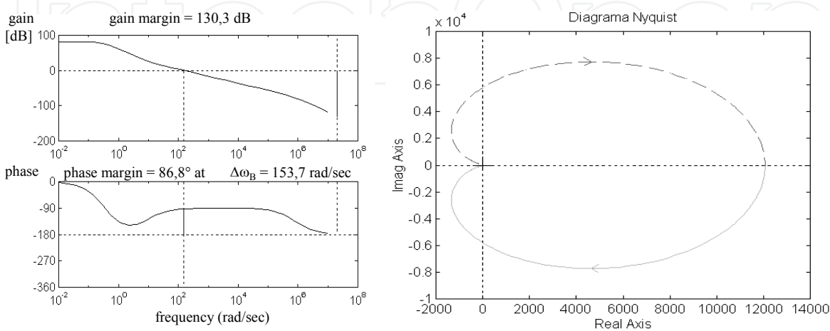
Fig. 11. Direct-loop transfer function of the weighted process in Bode and Nyquist diagram.
