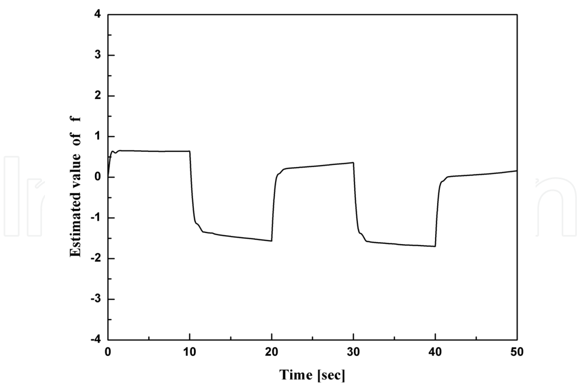
Fig. 11. Estimated value for the system uncertainties of the ABSC system for the square wave type reference input
