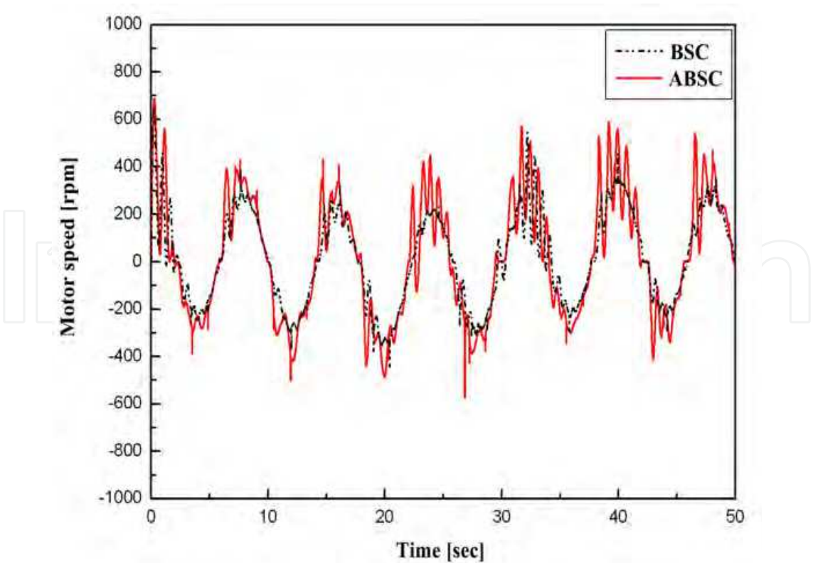
Fig. 9. Speed of the motor as the control input for the sinusoidal reference input
