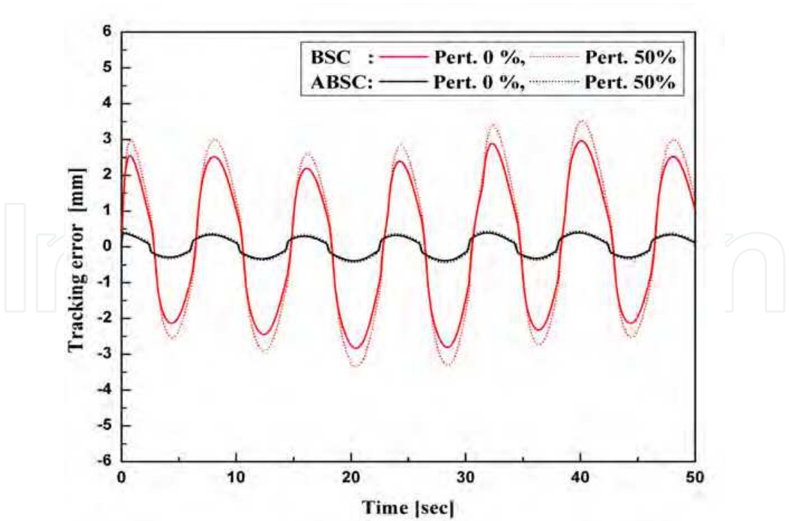
Fig. 5. Tracking errors of the BSC and ABSC systems with the perturbation of the system parameters
