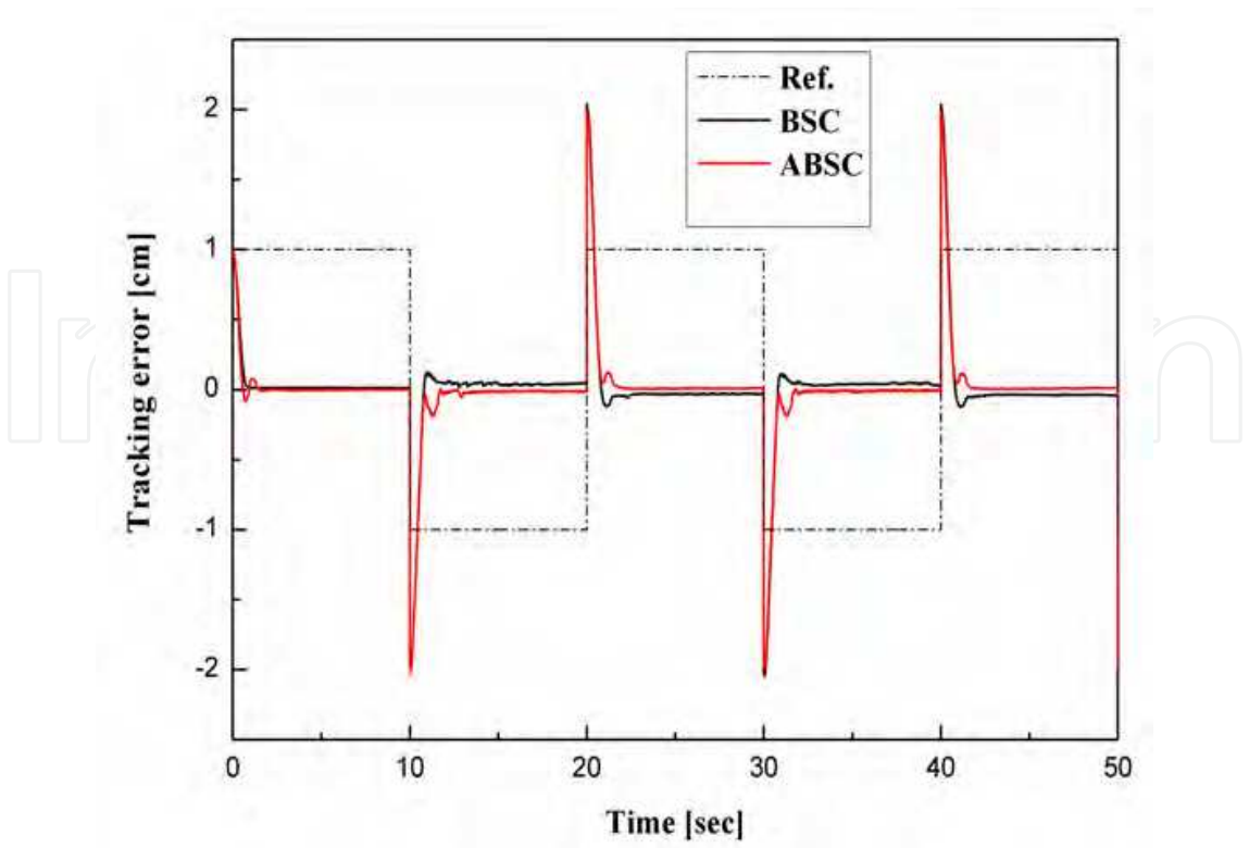
Fig. 10. Tracking errors of the BSC and ABSC systems for the square wave type reference input
