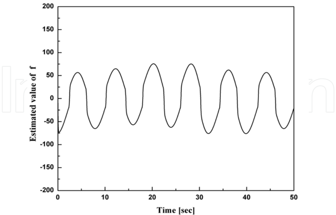
Fig. 4. Estimated value for the system uncertainties of the ABSC system for the sinusoidal reference input
