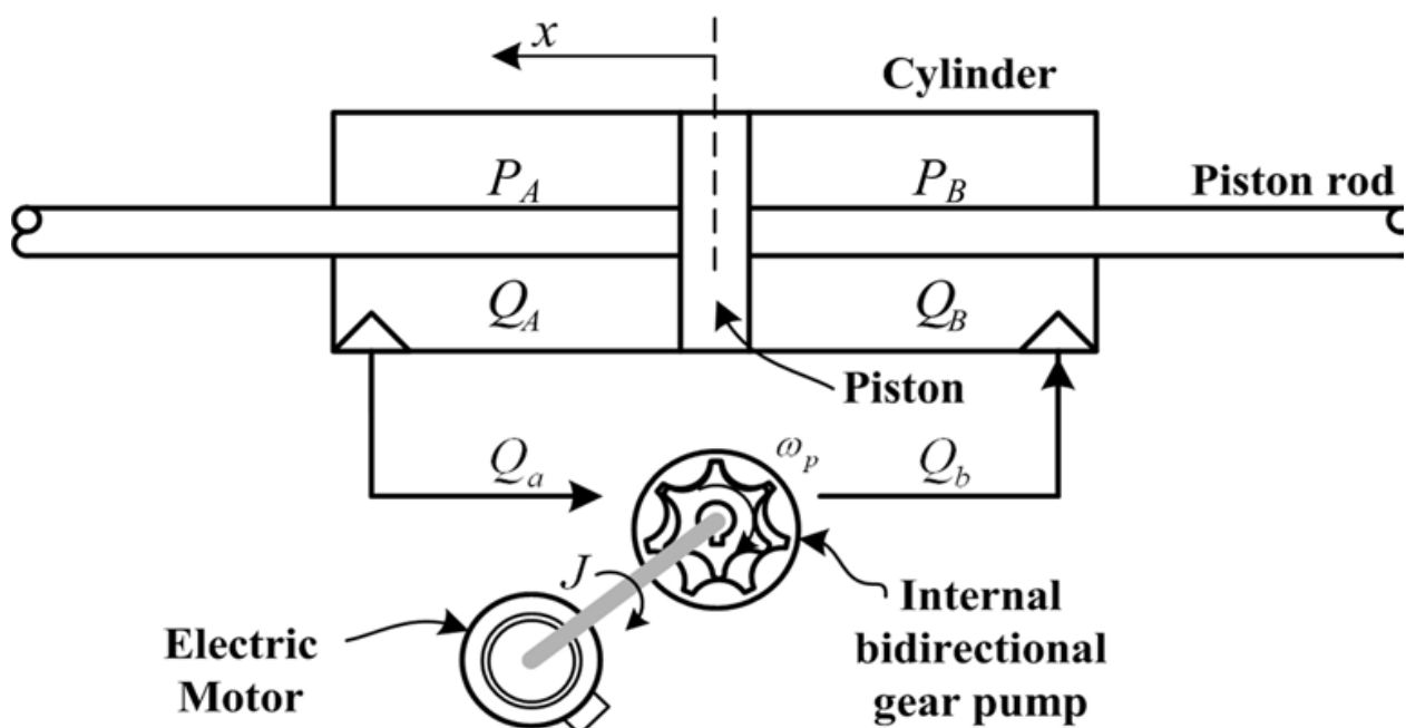
Fig. 1. Simplified schematic diagram of an EHA system
