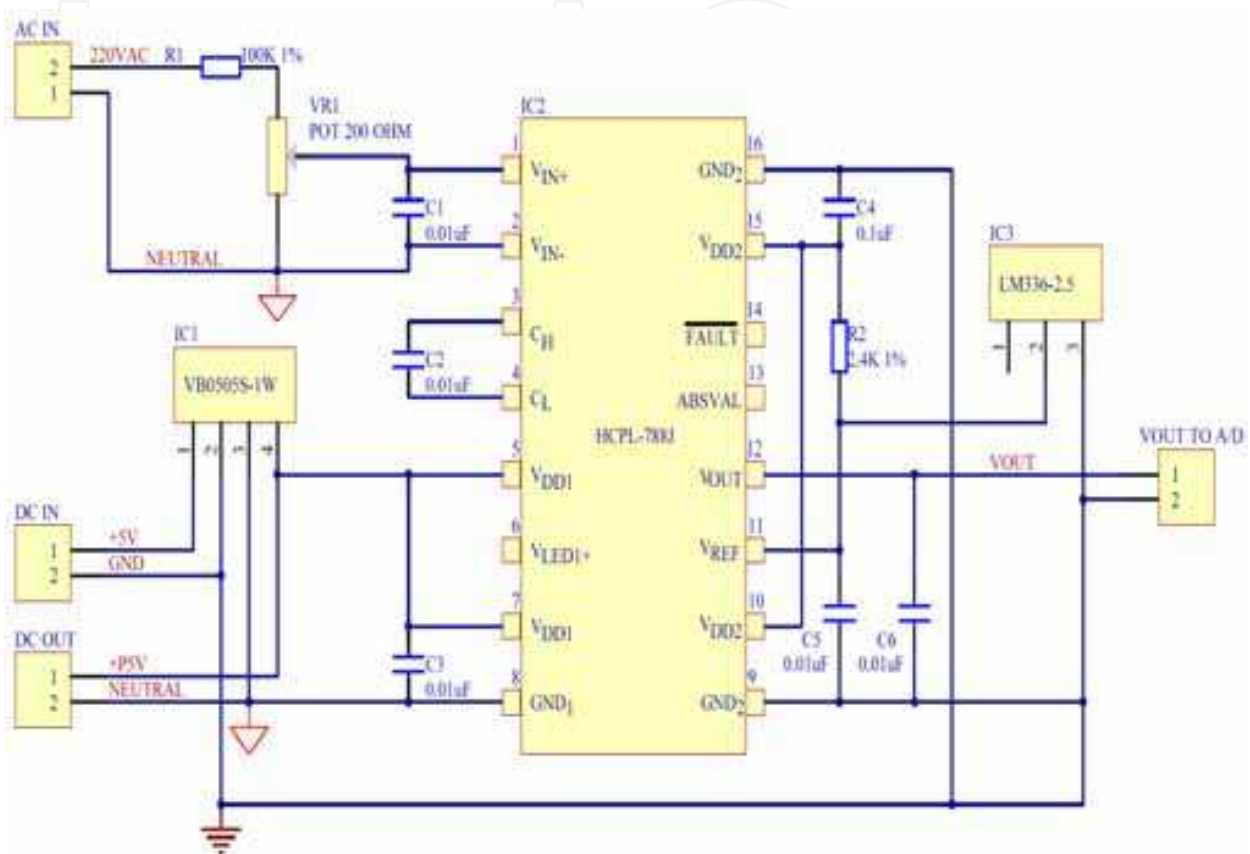
Fig. 2. The circuit of the signal conditioning module
