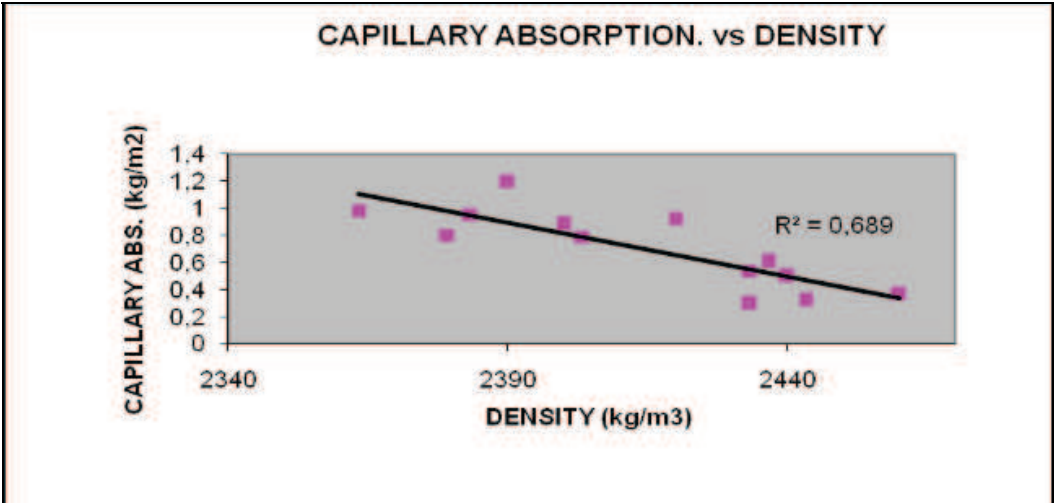
Fig. 4. Relation between capillary absorption and density
