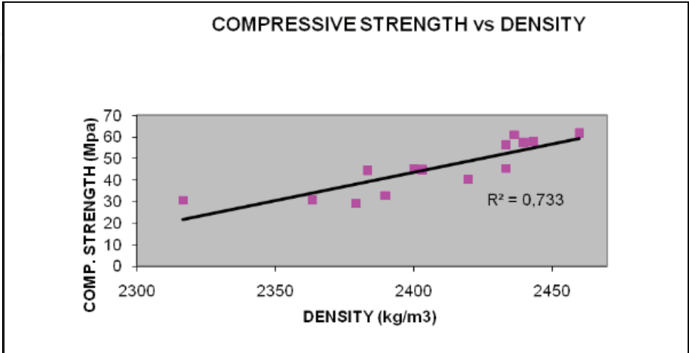
Fig. 5. Relation between compressive strength and density
