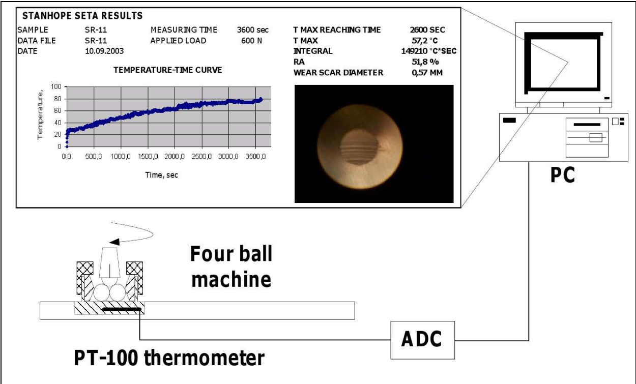
Fig. 6. Simplified scheme of the modified four-ball machine
