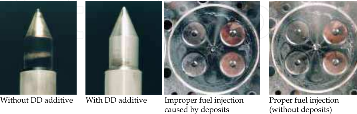
Fig. 1. Deposits on the injector Fig. 2. Effect of DD additives on the fuel injection
