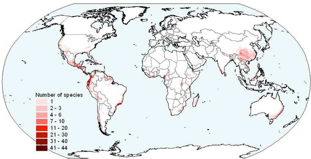
Fig. 2. Global distribution of threatened amphibians. Number of threatened species is shown in red. Important concentrations of threatened species are to be found from Southern Mexico to Ecuador and Venezuela, as well as the Greater Antilles, Atlantic Forests of southern Brazil, upper Guinea forests of western Africa, forests of western Cameroon and eastern Nigeria, Albertine Rift of eastern central Africa, Eastern Arc Mountains of Tanzania, Madagascar, western Ghats of India and Sri Lanka, Borneo and Philippines, eastern Australia, central and southern China (Extracted from IUCN, 2011; Copyright 2011 International Union for Conservation of Nature and Natural Resources Red List Unit).
