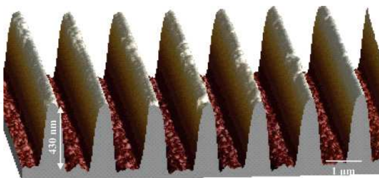
Fig. 5. Atomic force microscopy images of typical patterned surfaces of photochromic polymers. (Athanasios et al 2006a)
