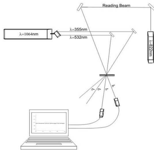
Fig. 10. Experimental setup for the measurement of the diffraction efficiency of the photochromic gratings (10% wt. SP in PEMMA) ( \lambda_{UV}=355\text{nm} , F_{UV}=20\text{ mJ cm}^{-2} , \lambda_{green}=532\text{ nm} , F_{green}=35\text{ mJ cm}^{-2} , \lambda_{reading\ beam}=822\text{ nm} .)
