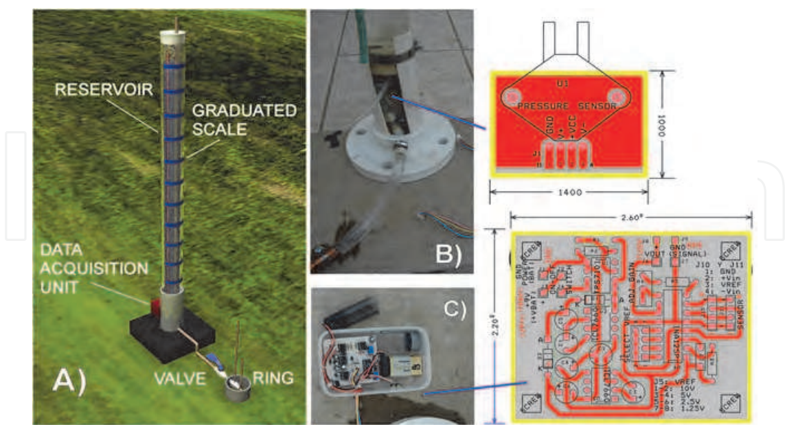
Fig. 14. A) Designed infiltrrometer. B) close-up of the pressure sensor assembly. C) The single- sided circuit is fitted into a small (2.6" X 2.2") printed circuit board fits into the plastic enclosure.
