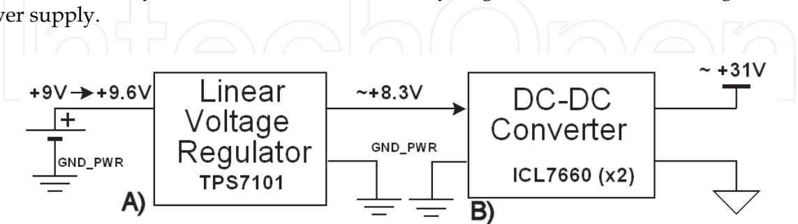
Fig. 5. Block diagram of the power supply. A) The battery feeds a linear voltage regulator. B) the output from the regulator is increased to (over) +30 V to power up the instrumentation amplifier.
