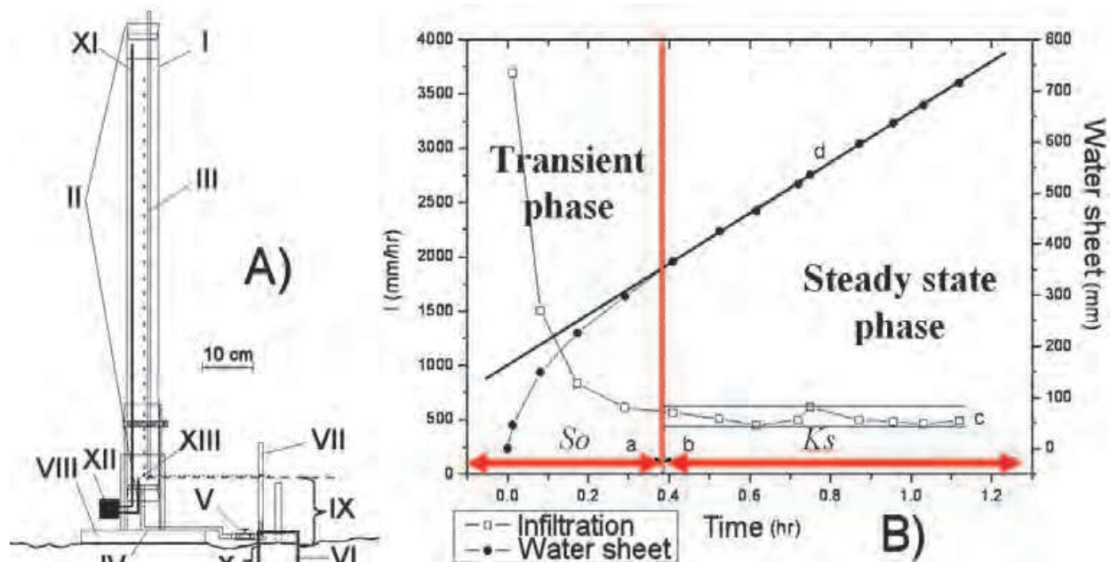
Fig. 1. A) Schematic diagram of an infiltrometer. I) Main reservoir (Mariotte), II) rubber stoppers, III) bubbling tubing, IV) water outlet, V) stop valve, VI) metallic ring, VII) purge and measurement of hydraulic load, VIII) stand base, IX) constant hydraulic load, X) insertion depth, XI) pressure sensor access to air chamber, XII) data logger, XII) pressure sensor access to the water column. B) Classical infiltration data results showing the transient and steady state phases of the infiltration process.
