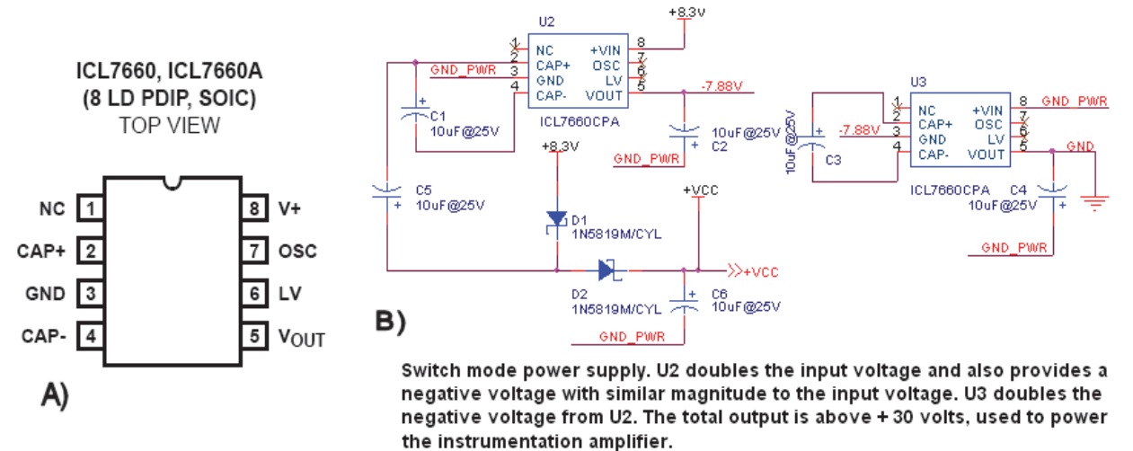
Fig. 7. A) Pinout of the ICL7660 CMOS converter. B) circuit diagram used to increase the TPS7101's output to ~+31V. Reproduced with permission. Copyright 2011 Intersil Americas Inc. All Rights Reserved
