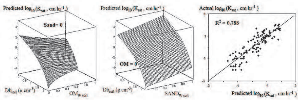
Fig. 1. Left and middle: 3-D visualisations of how log 10 Ksat varies with increasing soil bulk density (Db), sand fraction and organic matter (OM) fraction. Right: best-fitted log 10 Ksat versus actual data (right).
