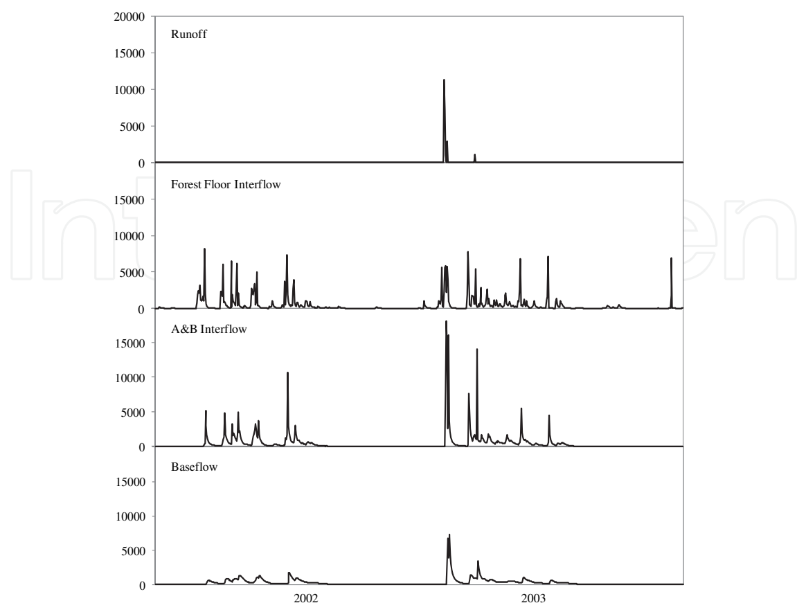
Fig. 5. ForHyM generated output for daily runoff, interflow (forest floor, A&B layers) and baseflow (in mm), for the Rithet River, BC. Basin details: Tables 3 and 4.
