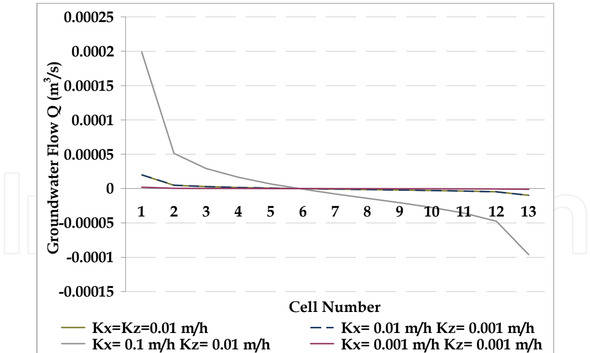
Fig. 10. Water flux between surface and ground on wetland-aquifer system.
