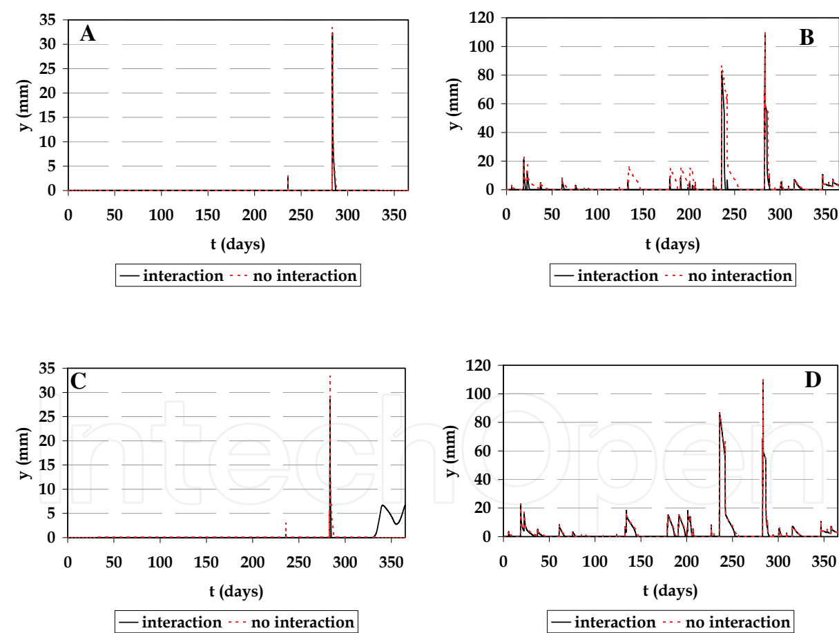
Fig. 6. Comparison of surface water depth on wetland section W4 with surface and groundwater interaction and with no surface and groundwater interaction (A) K_x=K_z=0.01 m/hr, (B) K_x=0.01 m/hr and K_z=0.001 m/hr, (C) K_x=0.1 m/hr and K_z=0.01 m/hr, (D) K_x=K_z=0.001 m/hr.
