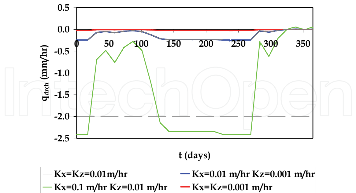
Fig. 7. Water flux between surface and ground on wetland section W4.
