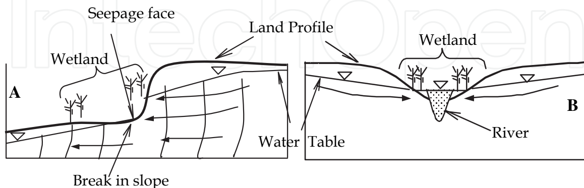
Fig. 1. Wetland and groundwater interactions: (A) Inflow from seepage faces and break in slope of water table. (B) Inflow to streams. (modified after Winter et al. , 1998)
